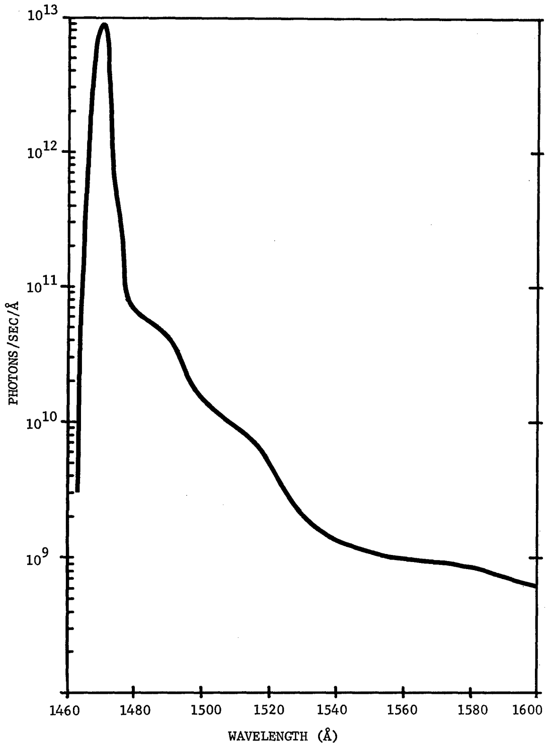
TYPICAL OUTPUT-PHOTONS/SEC/Å OF 582X XENON LAMP (RESOLUTION 7Å)
