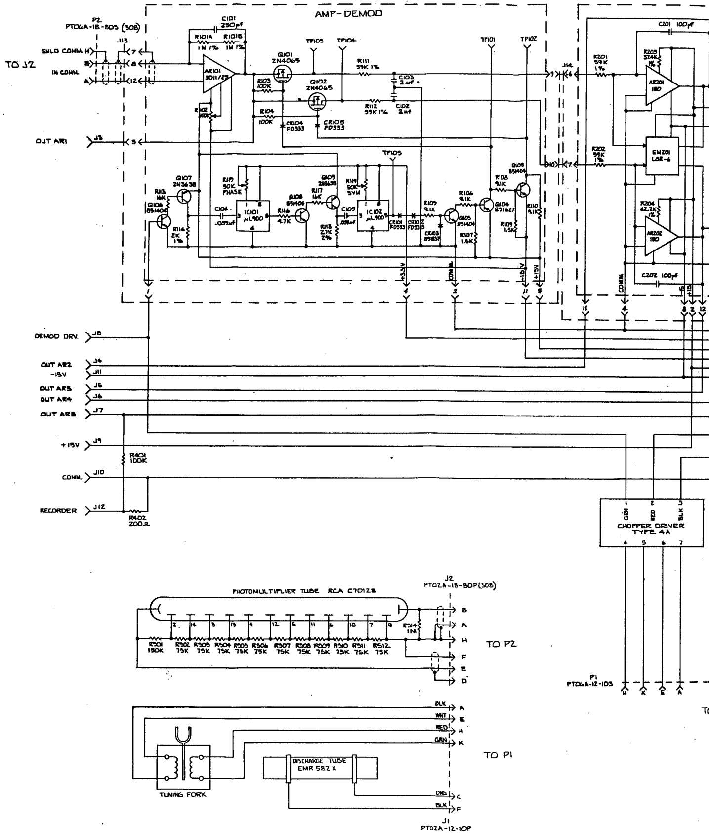
Figure 4. UV O 2 Sensor, Schematic Diag
