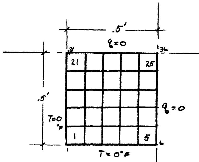
Figure A-2 Two Dimensional Heat Conduction
