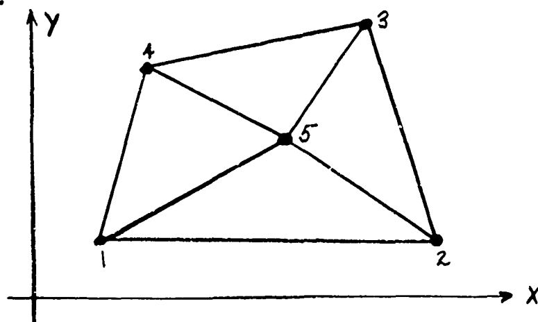
Figure 2-2 Quadrilateral Element
