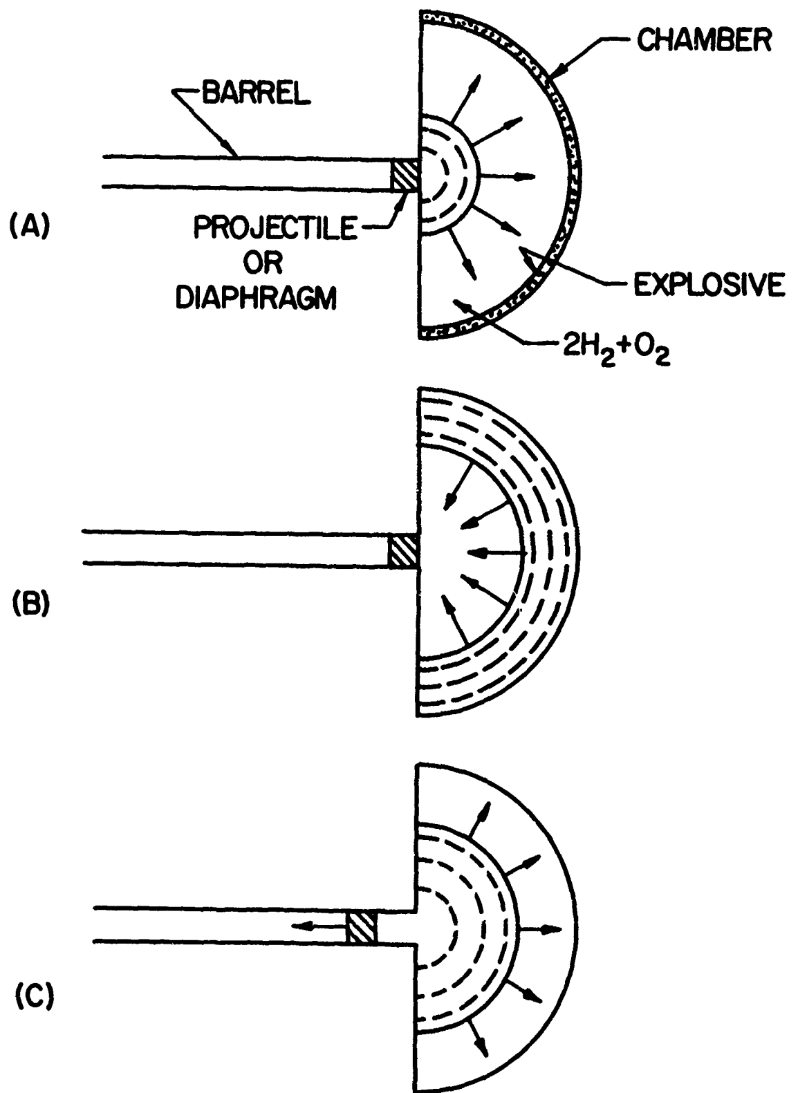
FIG. 1 SCHEMATIC OF PRINCIPLE OF OPERATION OF UTIAS HYPERVELOCITY LAUNCHER
