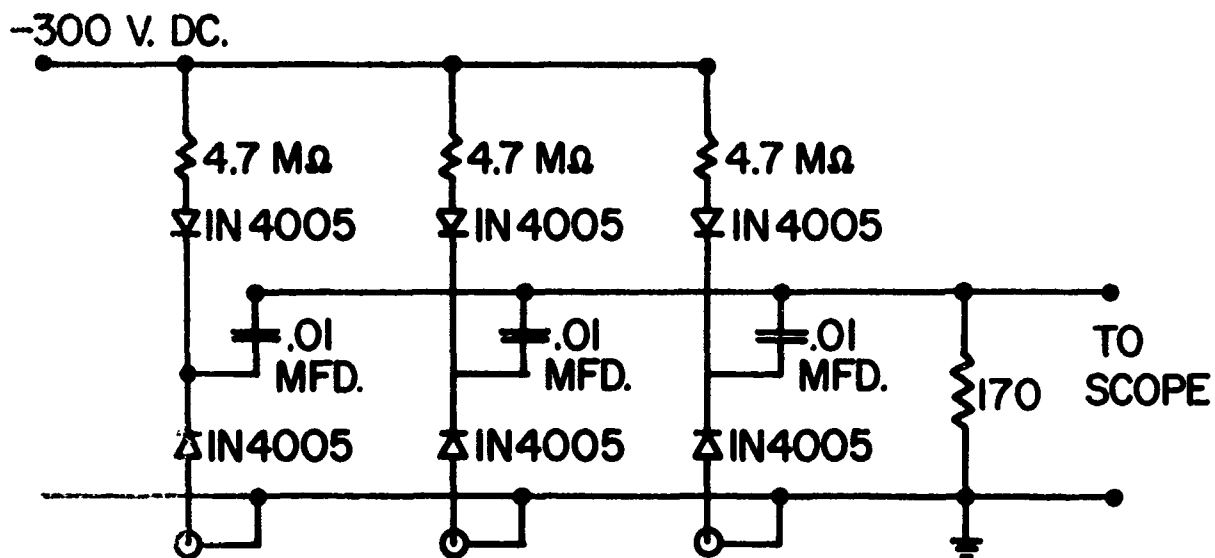
(B) IONIZATION PROBE CIRCUIT ACTUALLY USED
