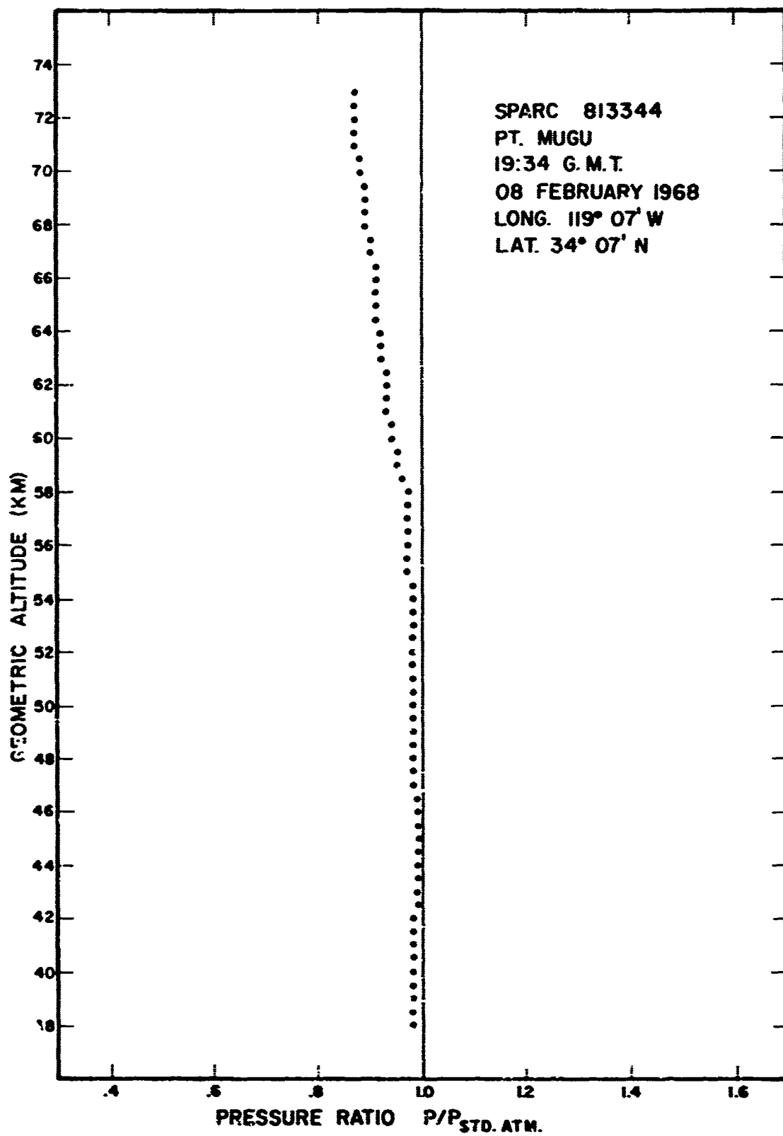
Figure 10. Altitude vs. pressure - Sparc 813344.
