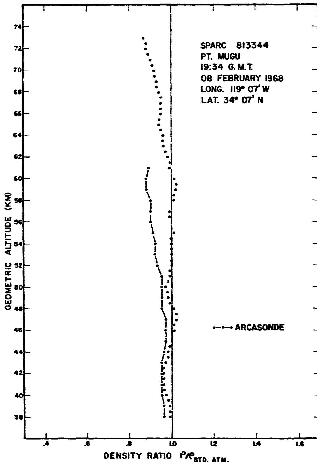
Figure 12. Altitude vs. density - Sparc 813344.
