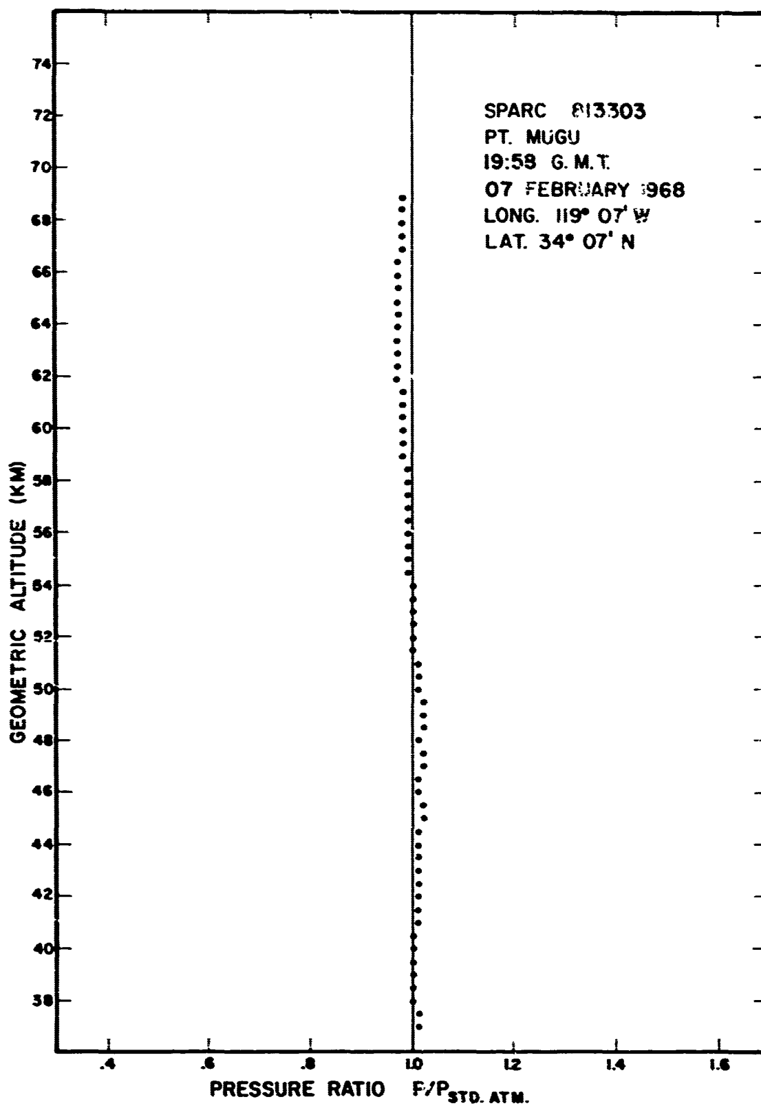
Figure 7. Altitude vs. pressure - Sparc 813303.
