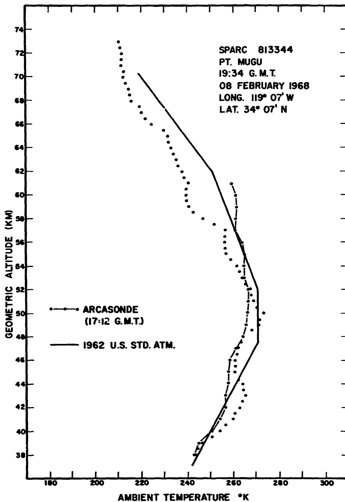
Figure 11. Altitude vs. temperature - Sparc 813344.
