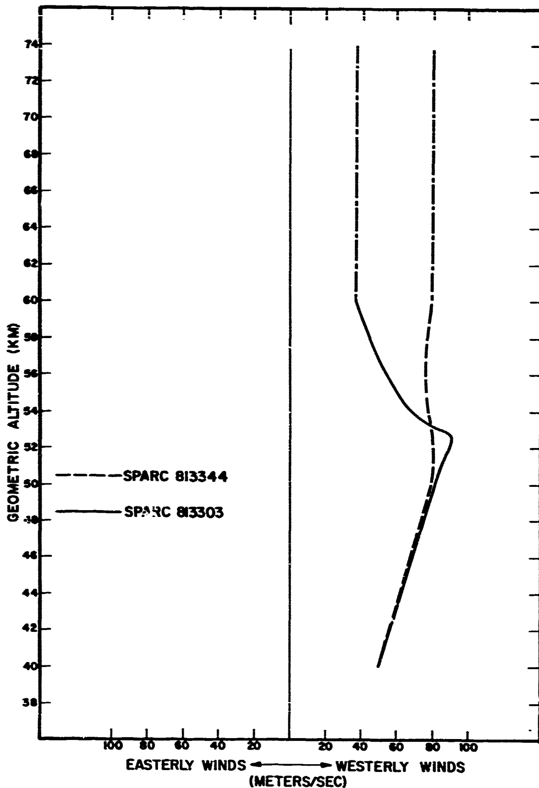
Figure 5. Zonal horizontal wind profiles.
