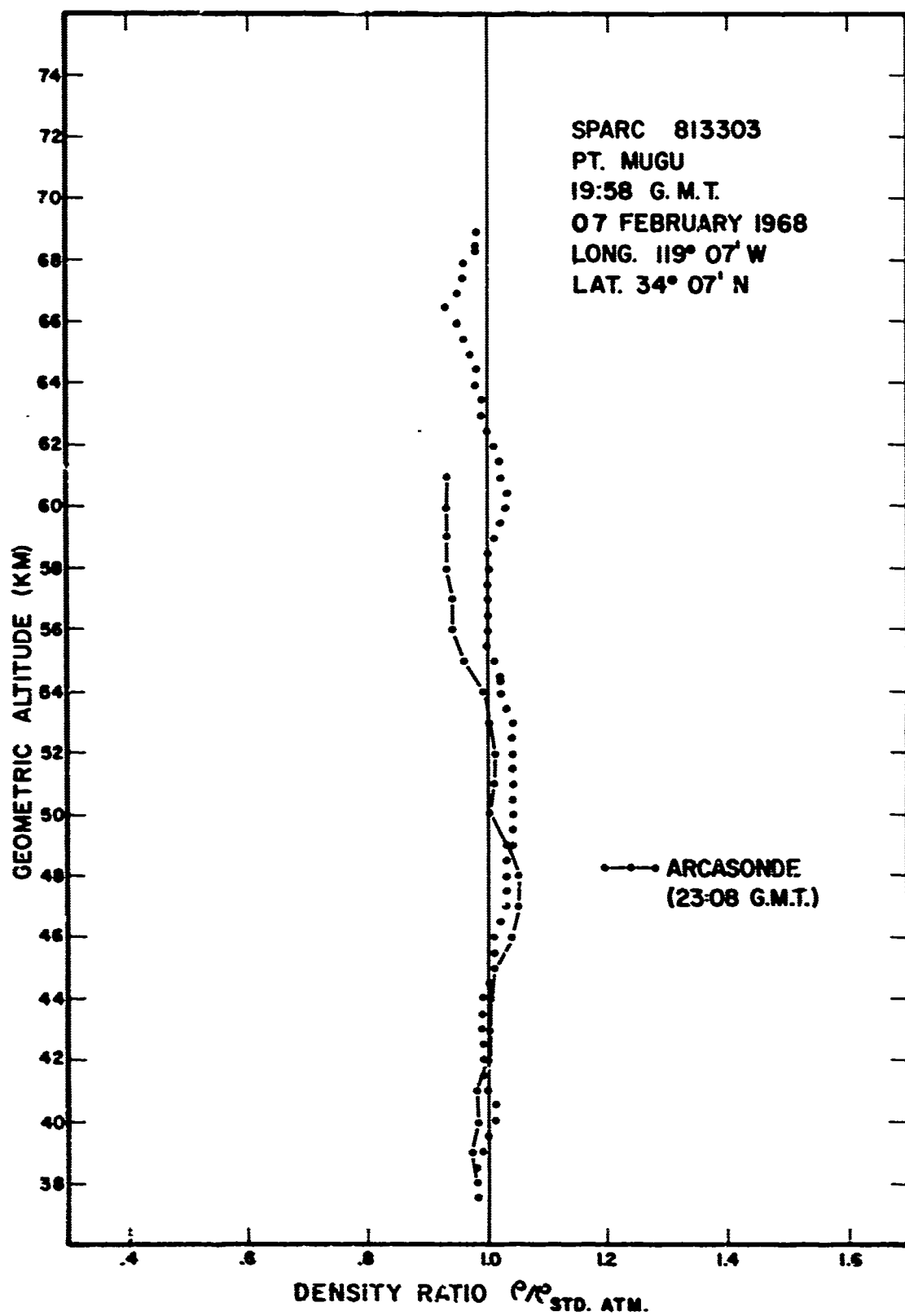
Figure 9. Altitude vs. density - Sparc 813303.
