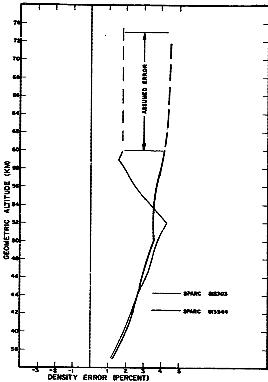
Figure 6. Density errors due to horizontal winds.
