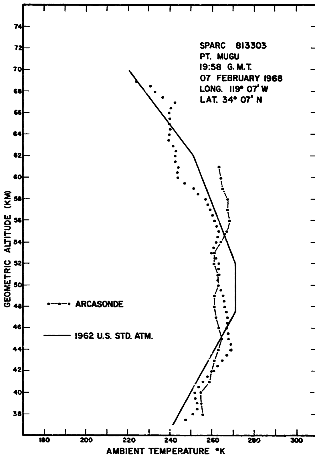
Figure 8. Altitude vs. temperature - Sparc 813303.
