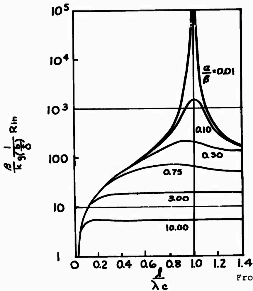
Figure 2-7. Resistance of Open-Ended Antenna
