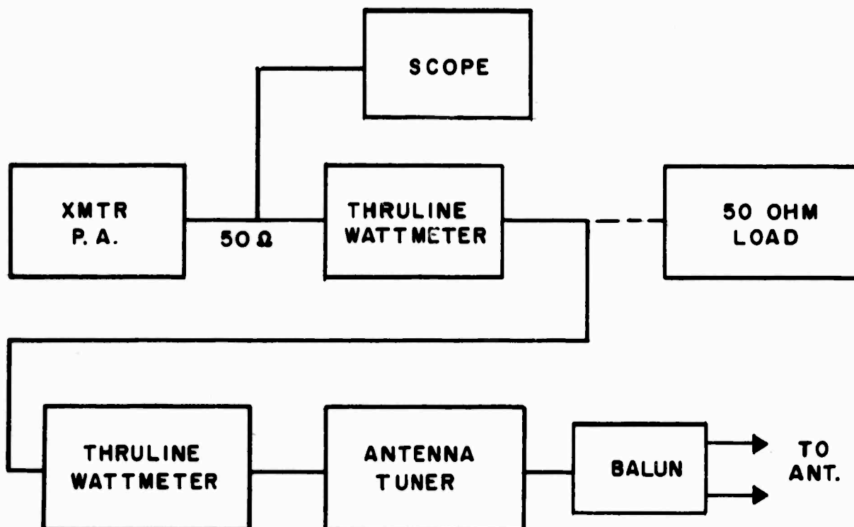
Figure 3-21. Transmitter Configuration.
