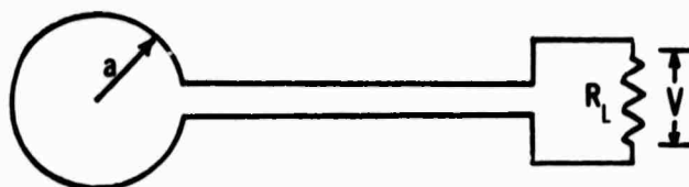
Figure 3-34. Balanced Receiving Loop.
