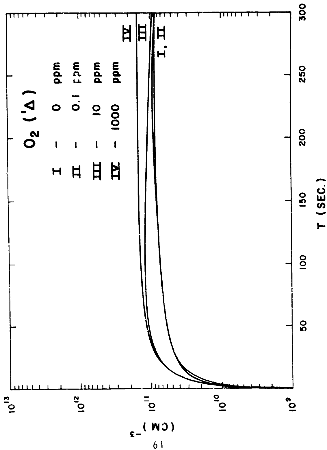
Figure 16. O_2(^{\circ}\Delta) Density Solutions During Interval 1 - 300 s
