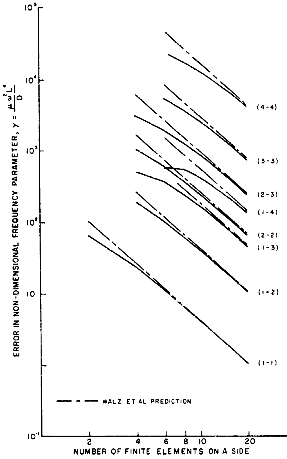
FIG. 8: COMPARISON OF WALZ, ET AL PREDICTIONS WITH ACTUAL ERRORS
