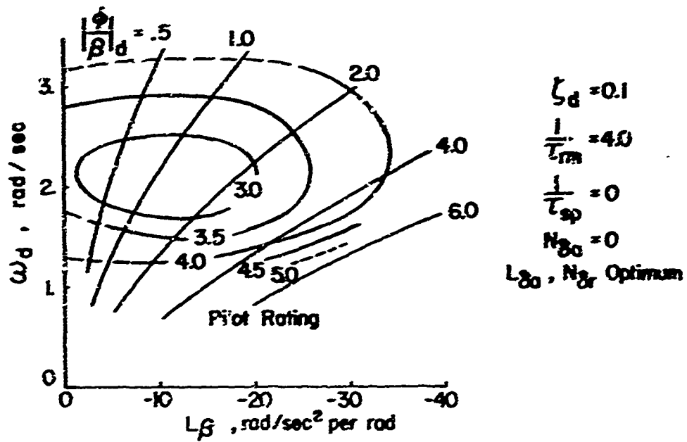
FIGURE 8 CONSTANT |\frac{\phi}{\beta}|_d SUPERIMPOSED ON PILOT RATING CONTOURS, \omega_d vs L_\beta
