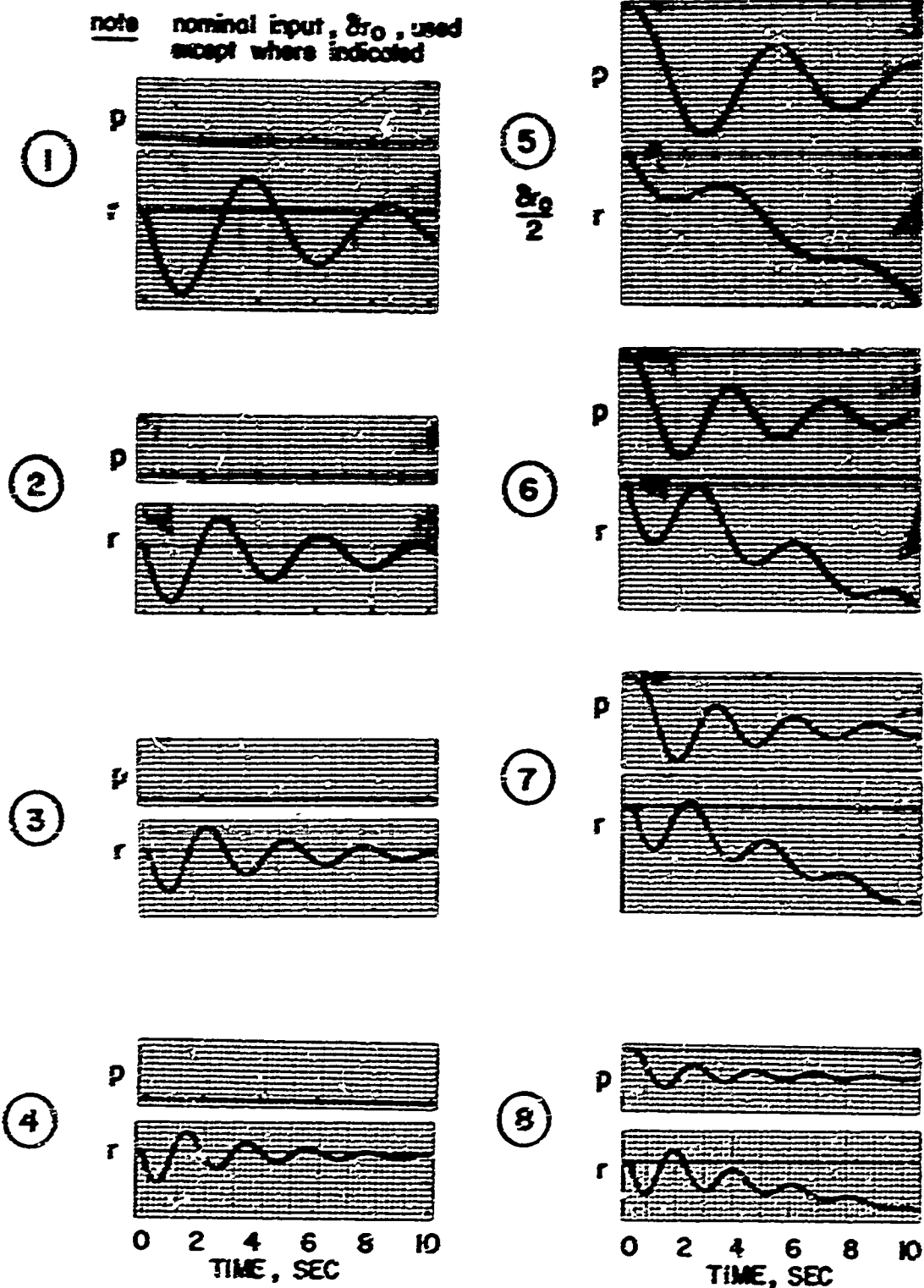
FIGURE 4 ANALOG COMPUTER ROLL RATE AND YAW RATE RESPONSES TO RUDDER STEP INPUTS
