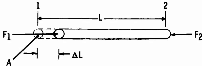
Figure 3-18. Tension/compression bar.
