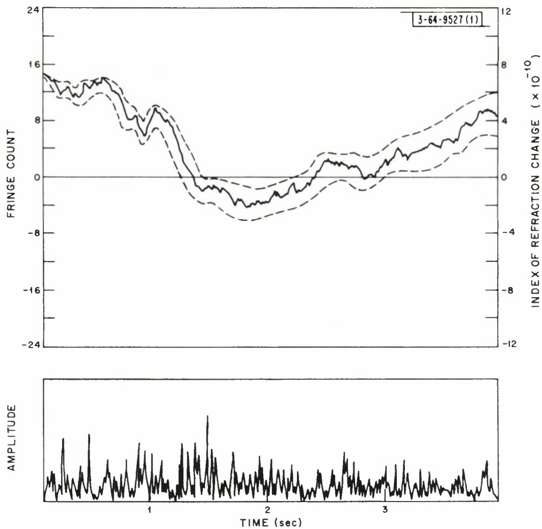
Fig. 3. Phase and amplitude for 29 July 1968 (1833 EST). Dashed curves show roughly the limits of expected phase error as a result of fades.
