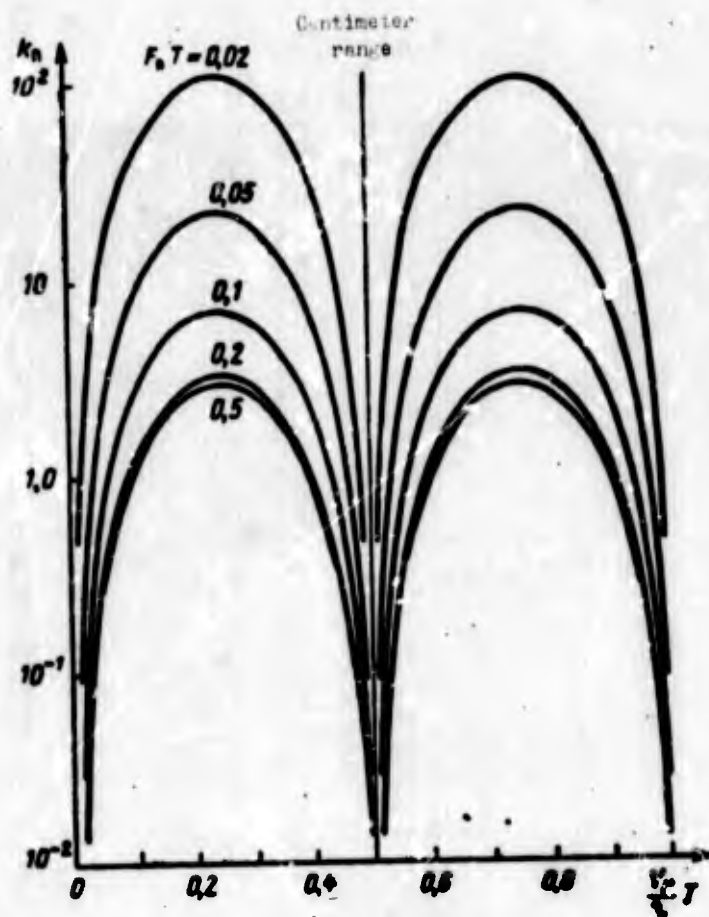
Fig. 7.19. The dependence of the coefficient of suppression by passive interferences of pulse-coherent radar in the centimeter range on the parameter \frac{v_r}{\lambda} T .
