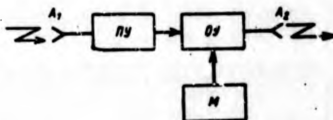
Fig. 8.7. Block-diagram of relay [retranslator] amplifier.
