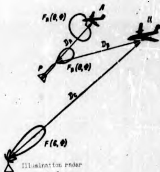
Fig. 8.2. A variant of the application of rocket-traps in a homing guidance contour of controlled antiaircraft rockets ZUR.
