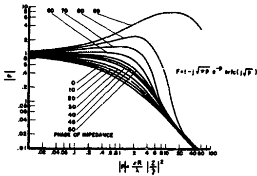
Magnitude of Sommerfeld's Attenuation Function
