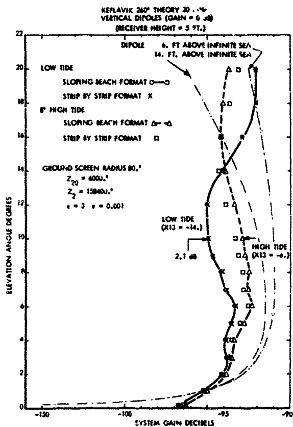
Figure 6. Predicted Power Gain for a Pair of Vertical Dipoles of 30 MHz Over Keflavik Naval Station 260° Profile
