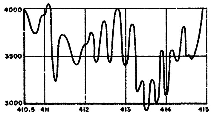
Fig. 4. EFFECTIVE PLASMA NOISE TEMPERATURE AT ANTENNA TERMINALS.
