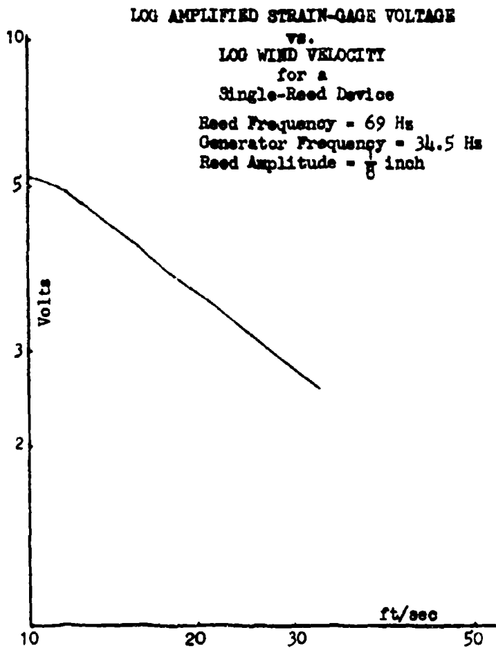
FIGURE 7. Constant-Driver-Coil-Current Plot.
