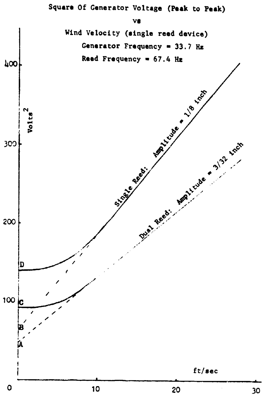
FIGURE 6. Constant-Reed-Amplitude Plots
