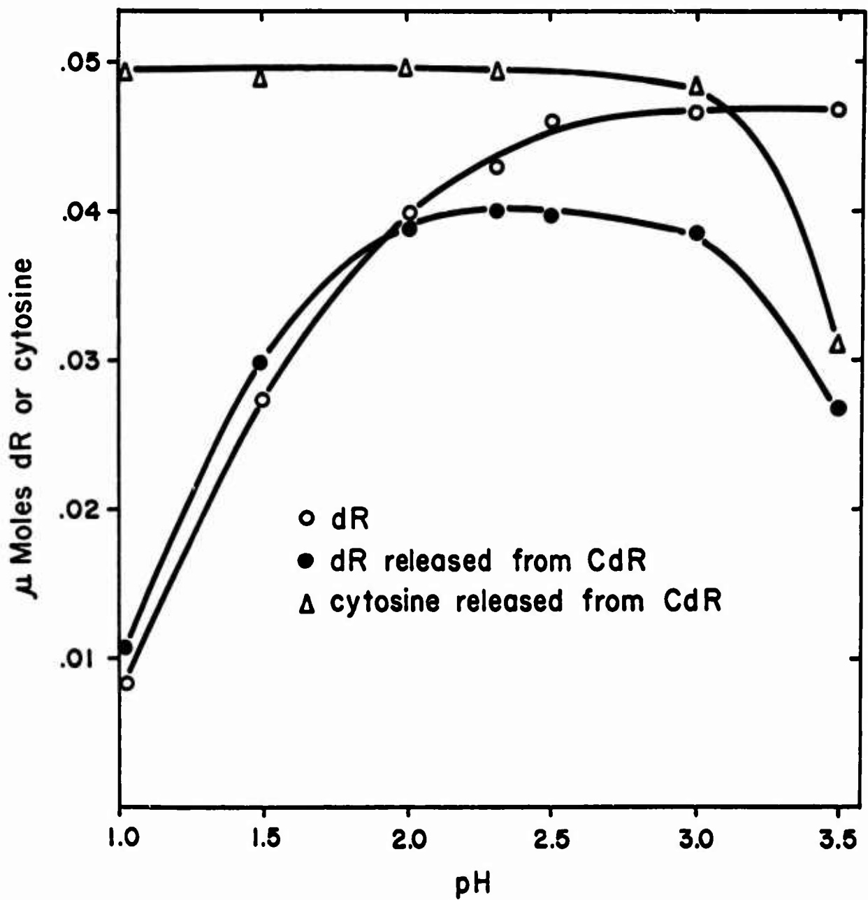
Figure B2 Effect of varying pH on the hydrolysis of CdR. 0.05 μmole each of CdR or dR was heated in 2 ml of HCl solutions with different pHs in a boiling water bath for 130 minutes. Amounts of dR and cytosine present at the end of the hydrolysis were measured as described in the text.
