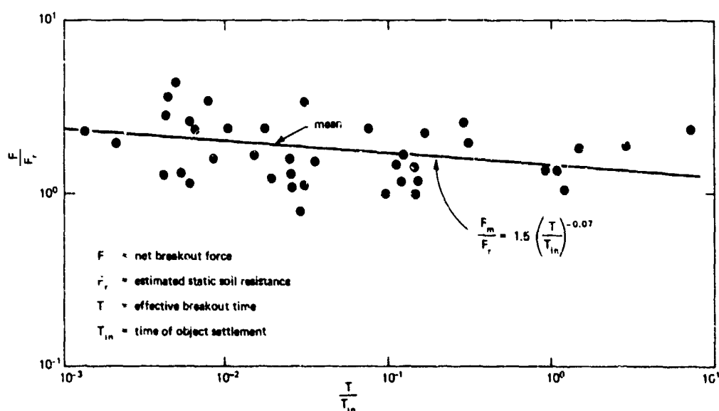
Breakout force versus time.
