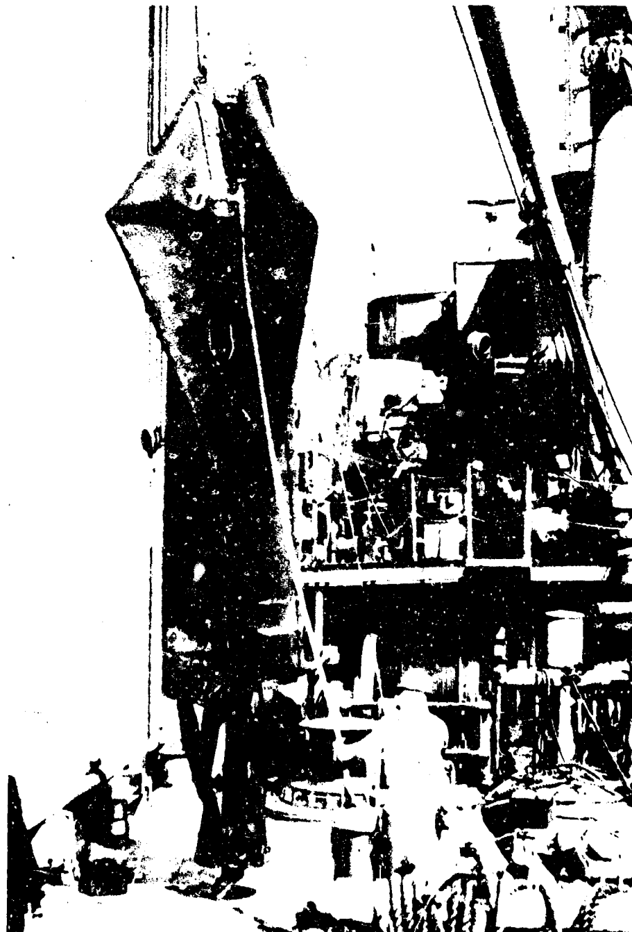
Collapsible salvage pontoon goes over the side for rigging and inflation.
