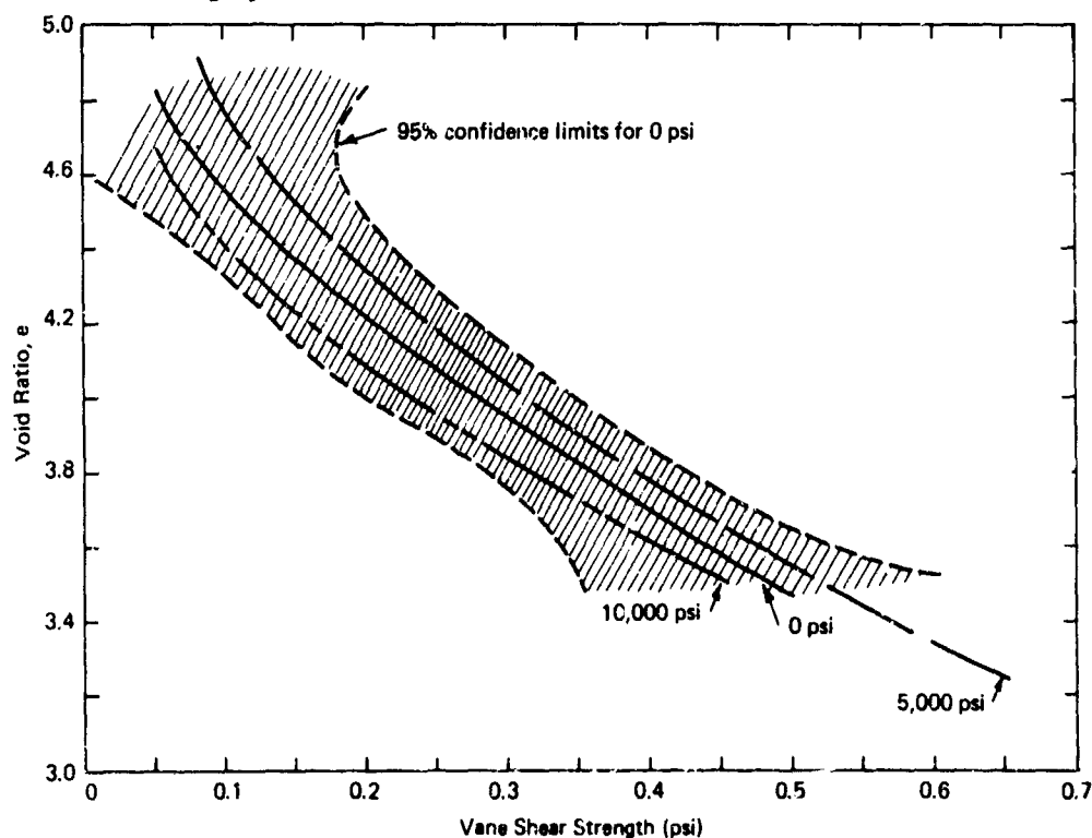
Quadratic regression fit to vane shear data for soil from 12,000-foot depths tested in pressure vessels.
