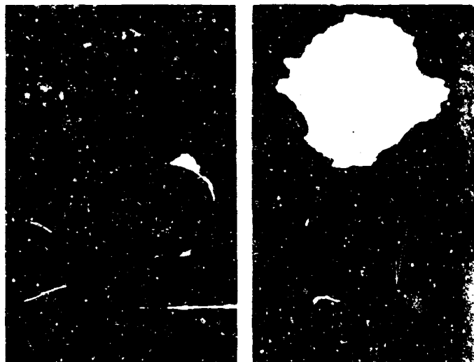
Crevice corrosion of precipitation hardened stainless steel exposed for 6 months at a depth of 5,640 feet. The specimen is shown before and after the bolt securing it has been removed.
