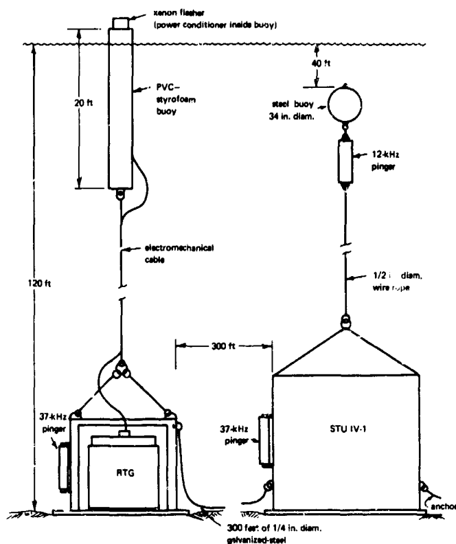
Shallow-water radioisotope thermoelectric generator emplacement.
