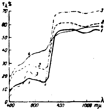
Fig. 4. Spectral curves for the reflection of desert vegetation. (According to Billings and Morris, 1951). 1 -- Atriplex canescens ; 2 -- A. lentiformis ; 3 -- Prunus andersonii ; 4 -- Eurotia lanata .
