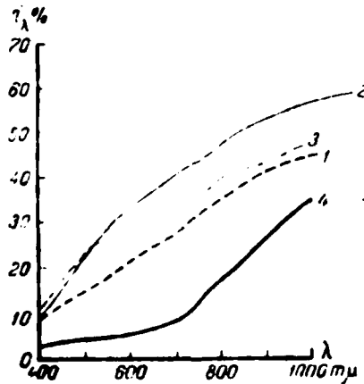
Fig. 6. Reflection spectral curves of soils. (According to Putseyko, 1945). 1 -- plowed soil; 2 -- meadow soil; 3 -- semiswampy; 4 -- swampy.
