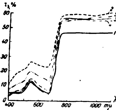
Fig. 5. Reflection spectral curves average for different habitat conditions. (According to Billings and Morris, 1951). 1 -- plains; 2 -- desert; 3 -- north slope pine forest; 4 -- west slope pine forest; 5 -- subalpine vegetation.
