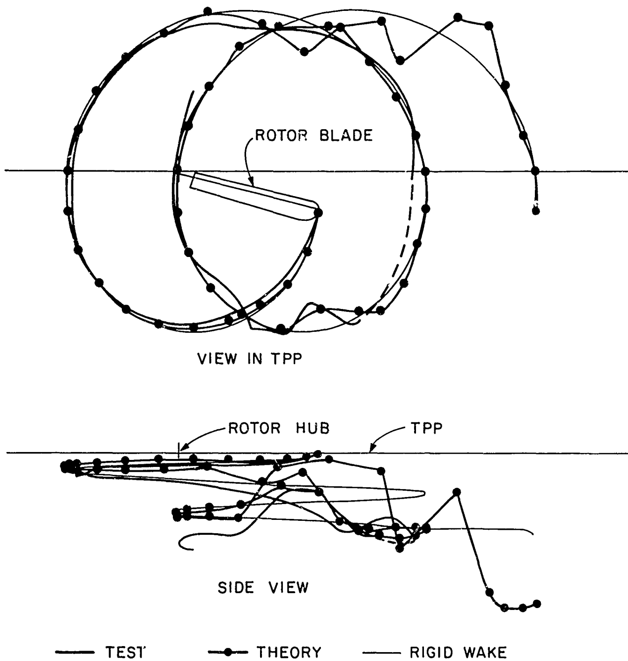
FIGURE 6 COMPARISON OF THEORY AND TEST RESULTS - n_1 = 2 , 3 rd ITERATION, \rho_c = 0.05 , \gamma_t = 1.0 , \gamma_s = 0.0 , AND \ell = 1.0
