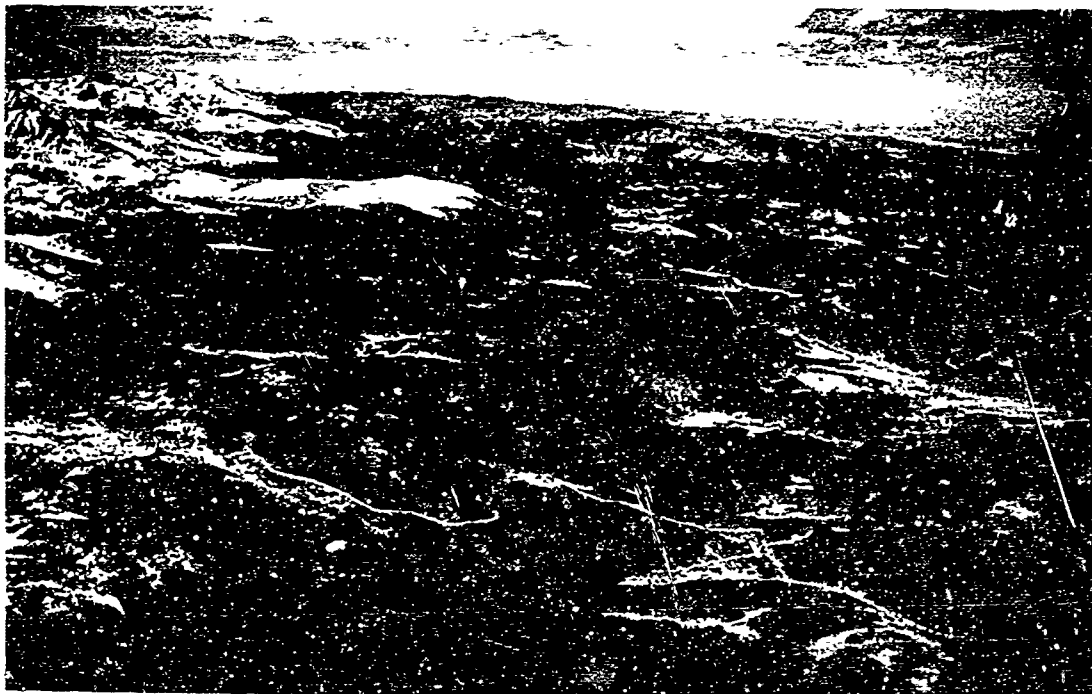
Figure 65. The Colorado Front Range and its eastern pediment
