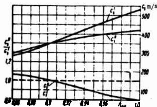
Fig. 4.20. Change of the gas exit velocity from jet nozzles of a ducted-fan engine during engine throttling ( H=0, M_0=0, y_p=1.73(p), T_{3(p)}=1300^\circ\text{K} ,
