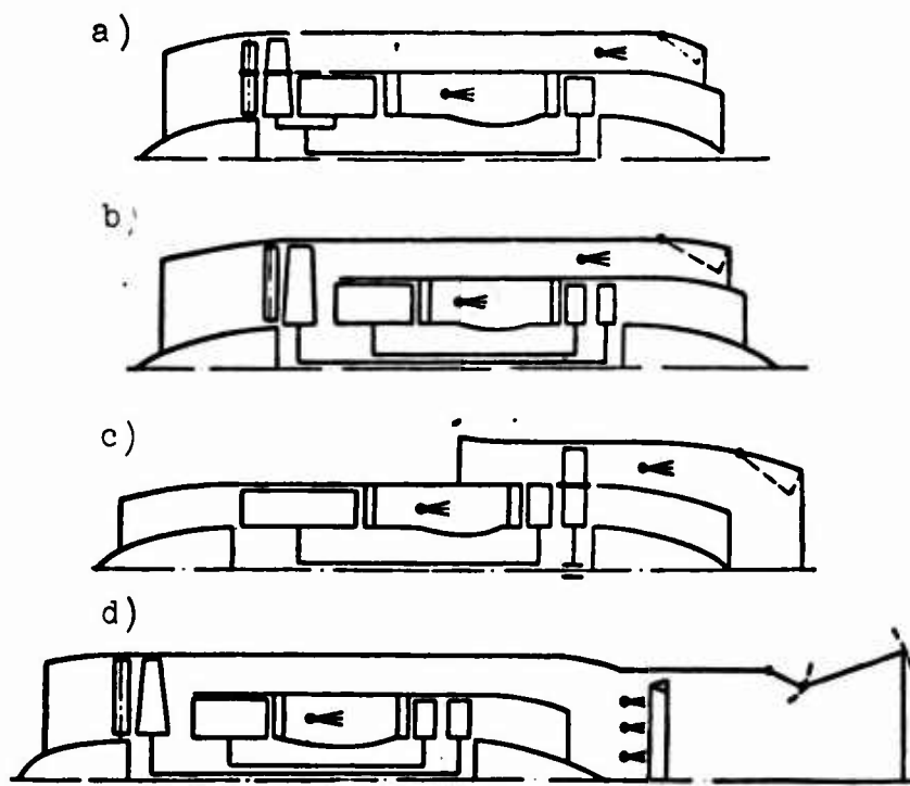
Fig. 1.3. Diagram of ducted-fan engines: a) single-shaft with separate exhaust; b) two-shaft with separate exhaust; c) two-shaft with aft location of fan; d) two-shaft with mixing chamber and afterburner.
