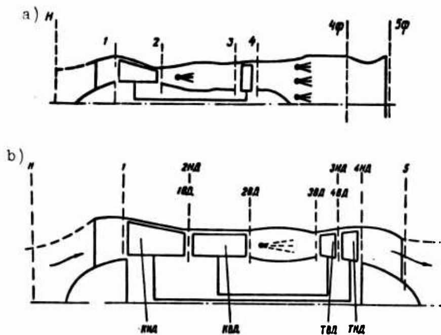
Fig. 1.2. Diagram of ducted-fan engines: a) single-shaft; b) two-shaft. [Translator's Note: HD = low pressure; BD = high pressure; KHD = low pressure compressor; KBD = high pressure compressor; TBD = high pressure turbine; THD = low pressure turbine].
