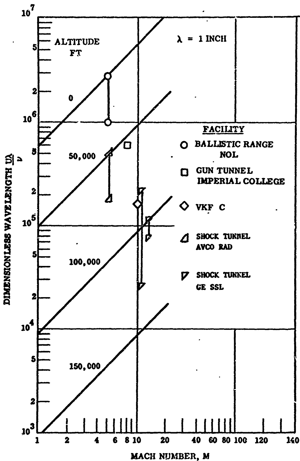
Figure 14. Dimensionless Wavelength in Flight and in Various Facilities for a Disturbance of Physical Wavelength of 1 Inch (Fechko 1968)
