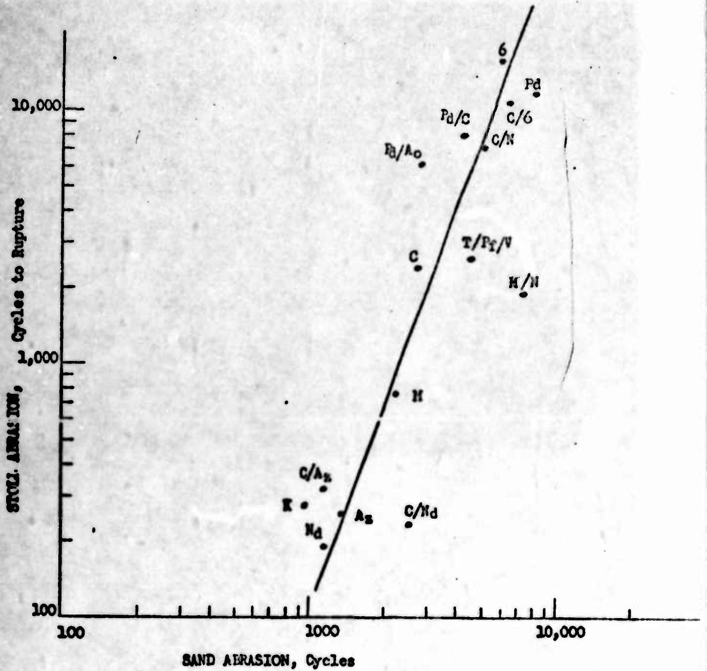
Figure 6. Comparison of Stoll and Sand Abrasion
