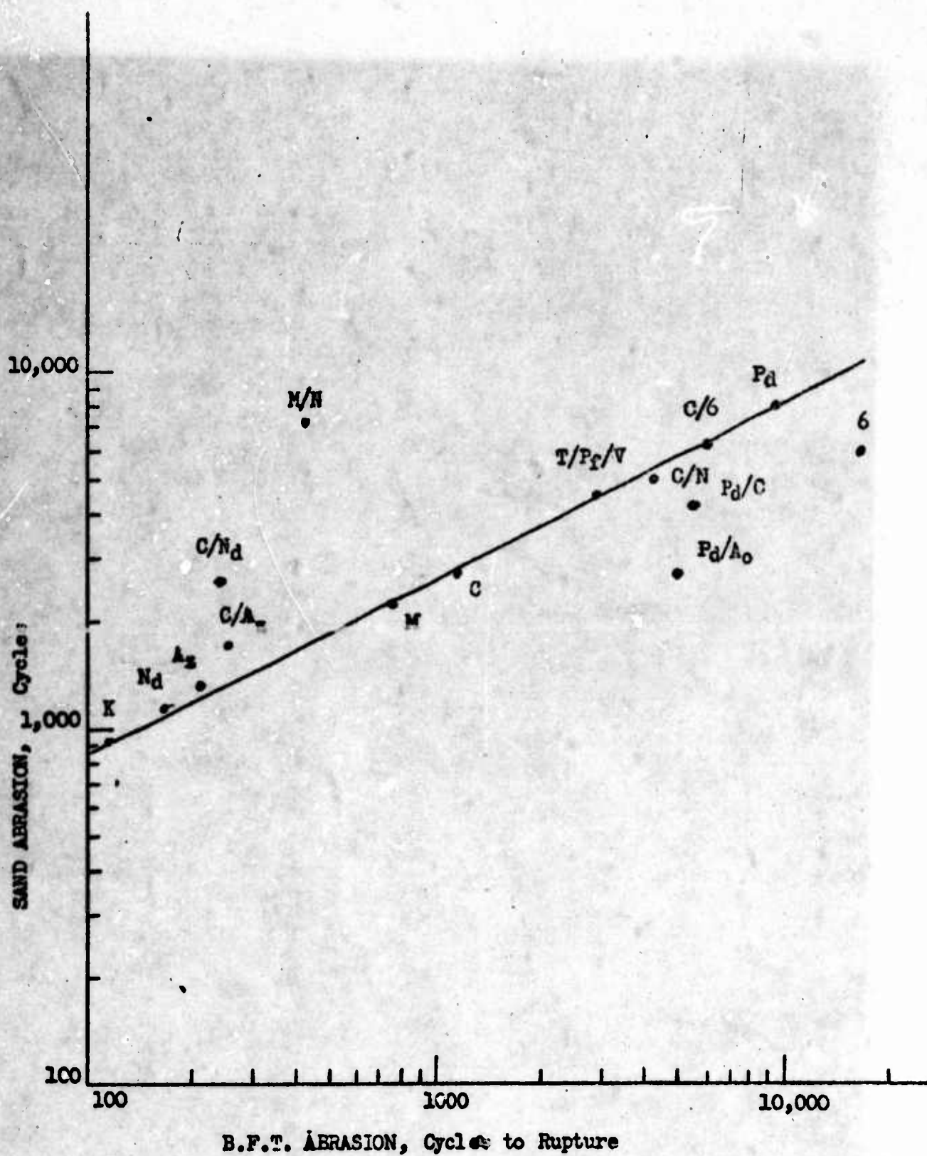
Figure 4. Comparison of Sand and BFT Abrasion
