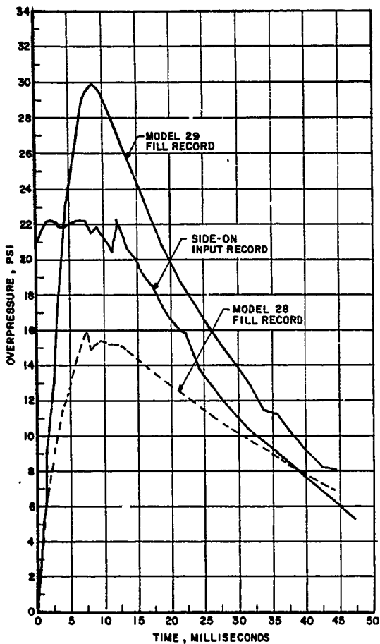
Figure 17. Comparison of Filling Through Single and Multiple Entrances - P_s = 21 psi
