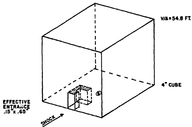
(A) MODEL 17- BAFFLE IN ENTRYWAY
