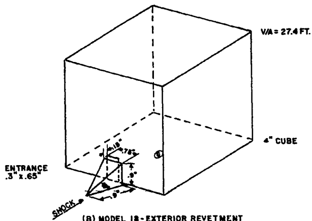
(B) MODEL 18-EXTERIOR REVETMENT
