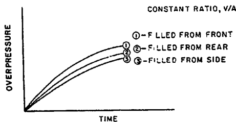
(B) EFFECT ON FILLING BY MODEL ORIENTATION
