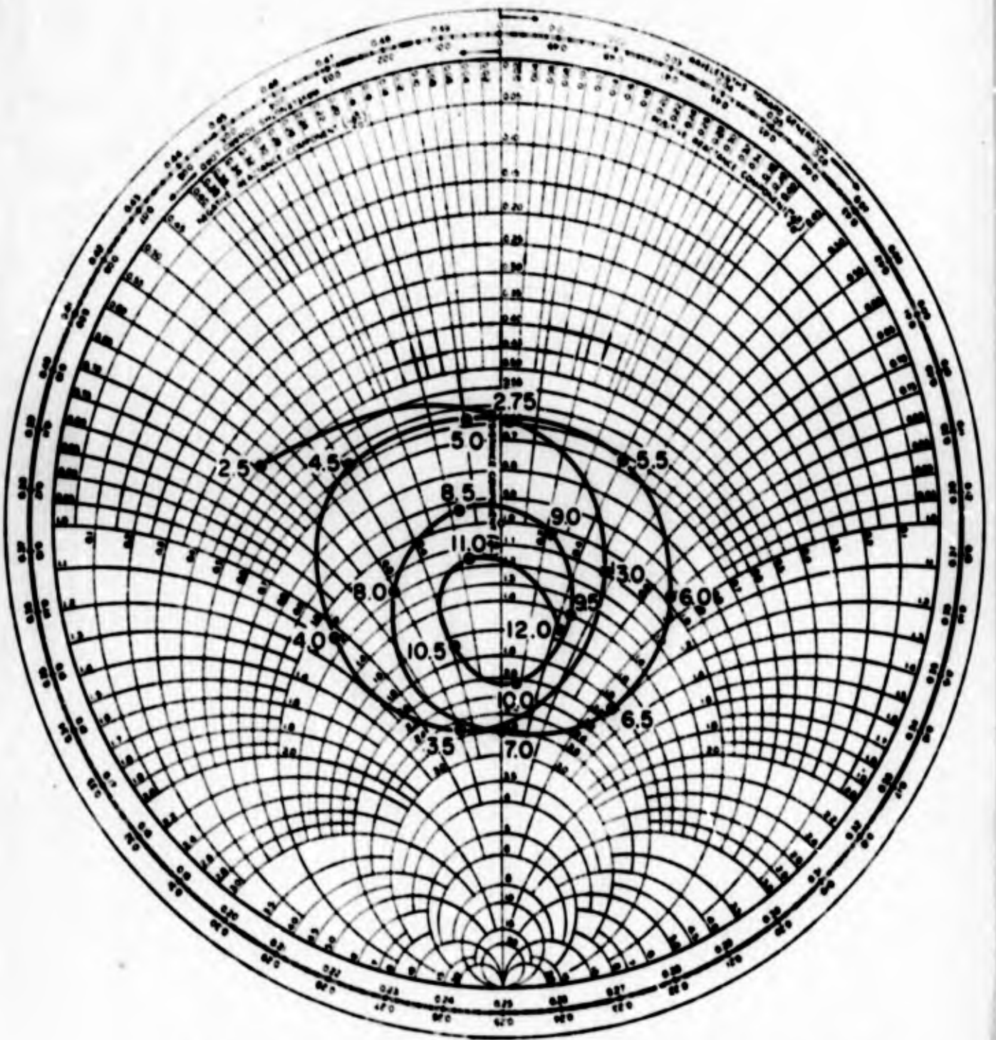
Fig. 4 - Conical Monopole Antenna Impedance Relative to 50 Ohms (0.196 \lambda at 2.75 Mc transformer of 70 ohm line)
