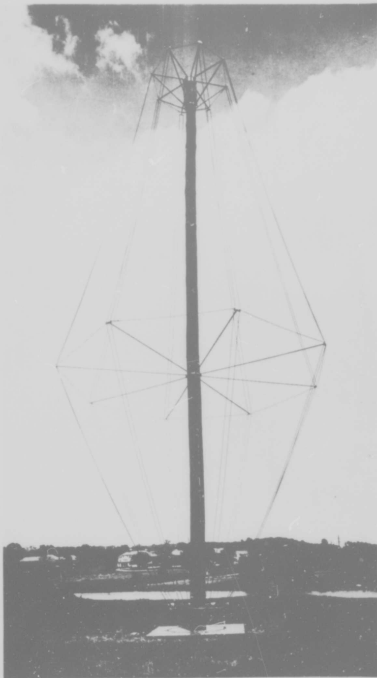
Fig. 2 - Conical Monopole Antenna 2.75 to 11.0 Mc 57 Feet High
