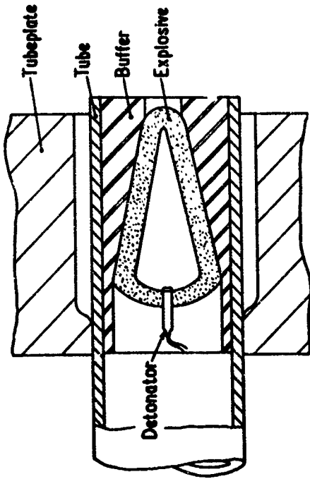
Figure 12. Schematic for Explosion Welding Tube to Tubeplate Using a Supersonic Detonation Rate Explosive and a Tapered Buffer (4).
