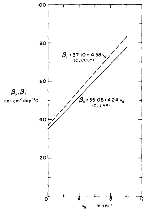
Figure 3. Slopes in eq 10-15 as functions of windspeed.
