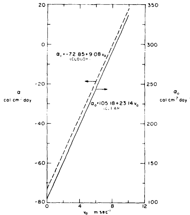
Figure 2. Intercepts in eq 10-15 as functions of windspeed.
