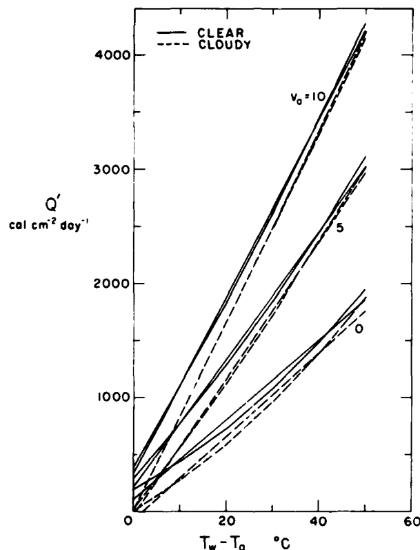
Figure 1. Total heat-loss rate, neglecting short-wave radiation, as a function of T_w - T_a , with windspeeds at 0, 5 and 10 m sec -1 .
