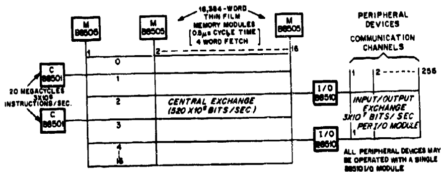
Figure 3--Modular data processors
