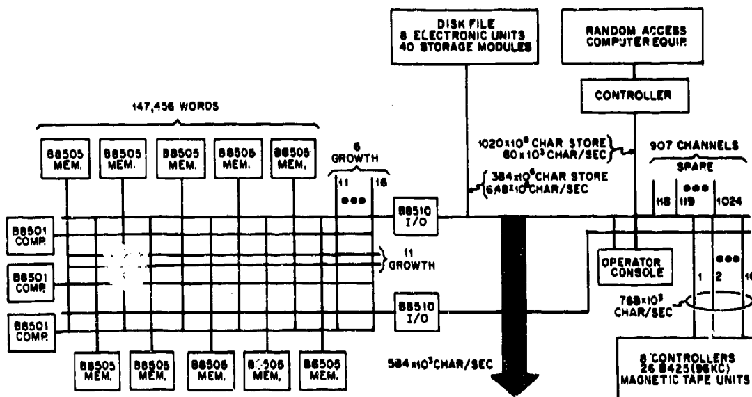
Figure 2—Further expanded B8500 system
