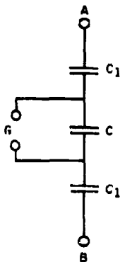
Fig. 2--Equivalent circuit of gas discharge display cell
