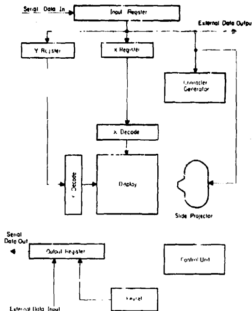
Figure 1 - Proposed PLATO IV terminal
