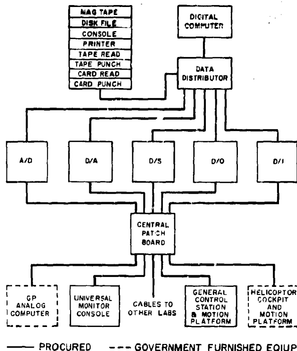
Figure 1 - Naval Training Device Center Research Tool Digital Computer System
