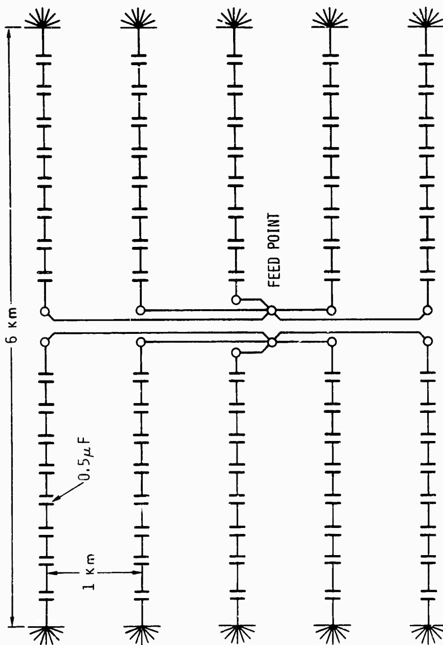
FIG. 9. VLF Transmitting Antenna Constructed Over Hawaiian Lava Beds.
