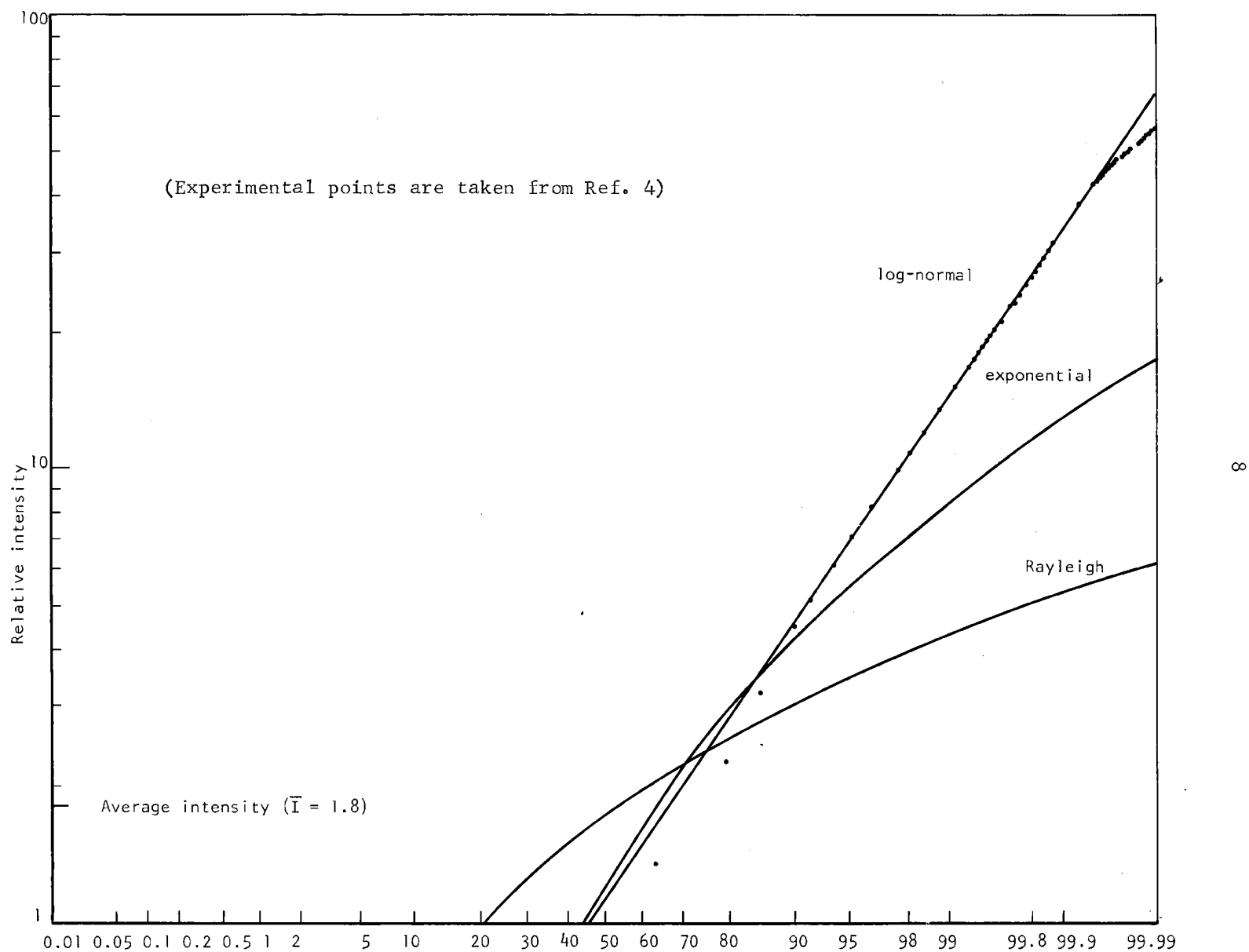
Fig. 1--Cumulative log-normal, exponential, and Rayleigh distributions with equal means
