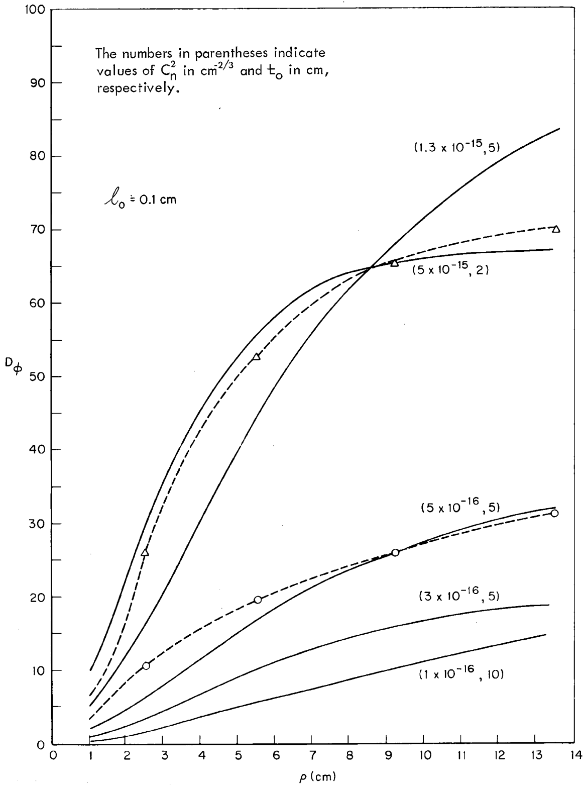
Fig. 3--Comparison of computed phase structure function with data of Bertolotti, et al., at a range of 3.5 km
