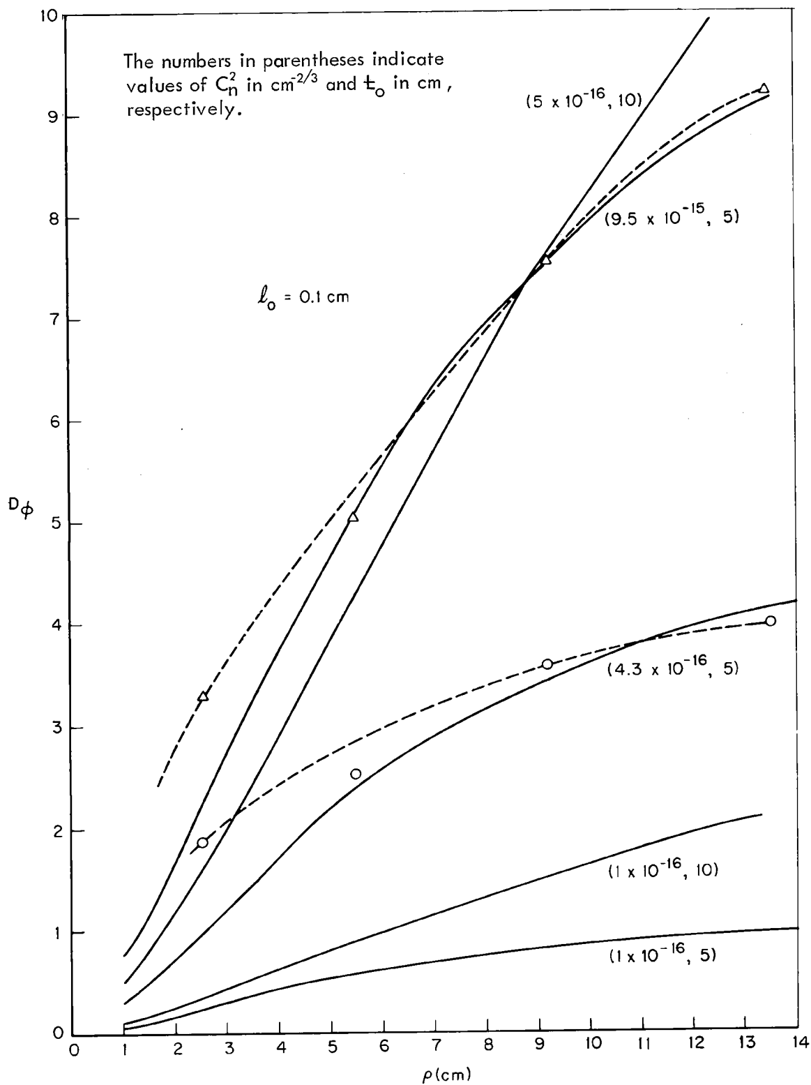
Fig. 2--Comparison of computed phase structure function with data of Bertolotti, et al., at a range of 0.5 km
