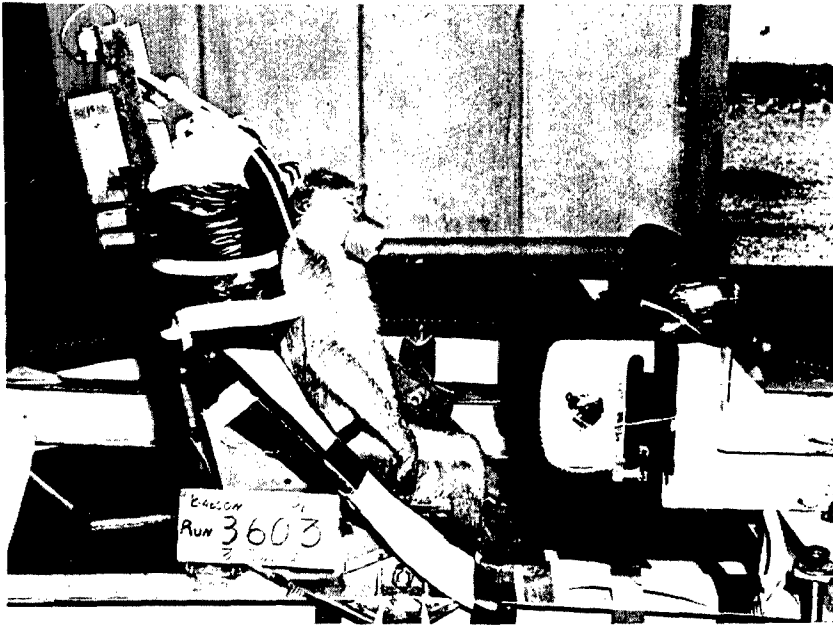
Fig. 6 - Airbag restraint system in position prior to run. Note that restraint over back of seat is released 6 secs prior to impact, and masking tape about chest breaks. Both hold animal in normal seated position during run, but are released at impact
