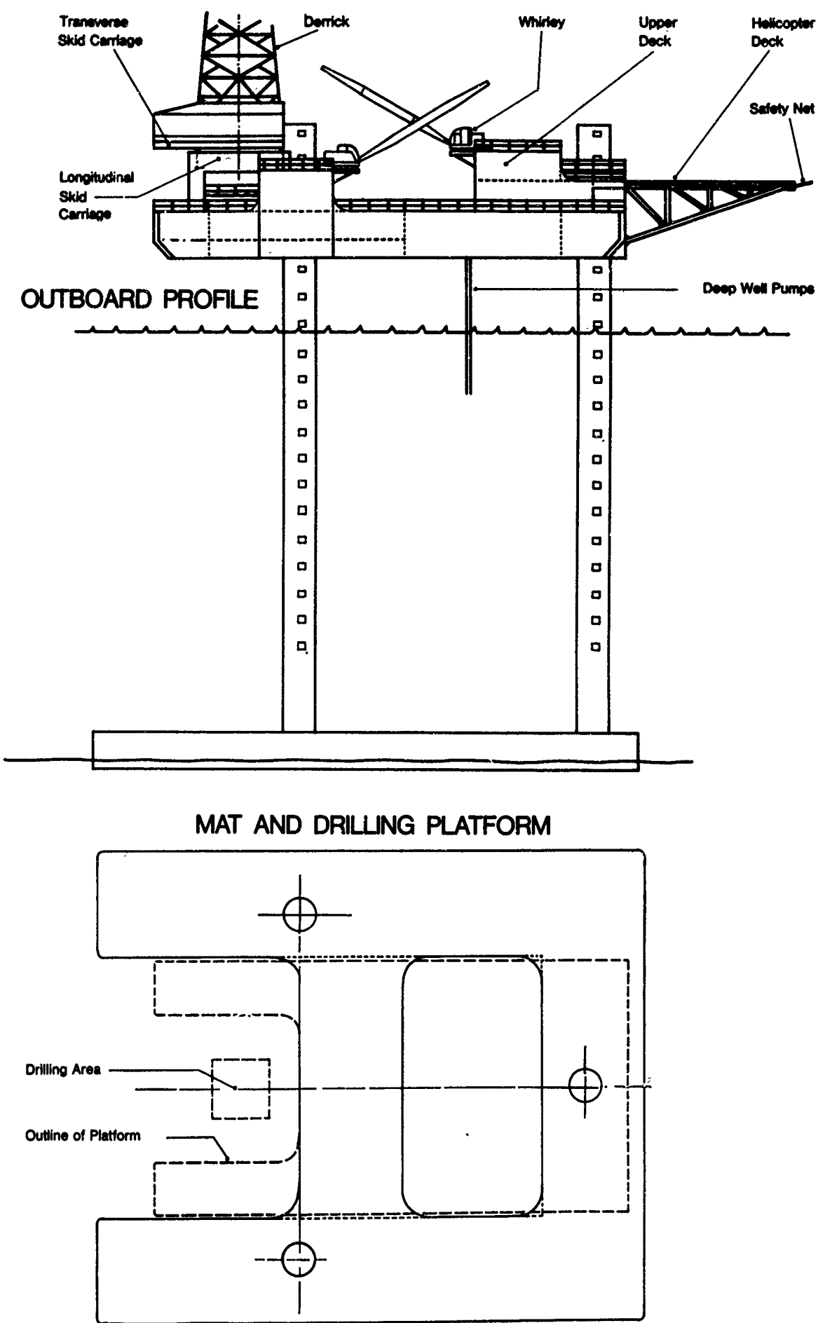
Figure 6.15 Schematic of mat-type jack-up.
