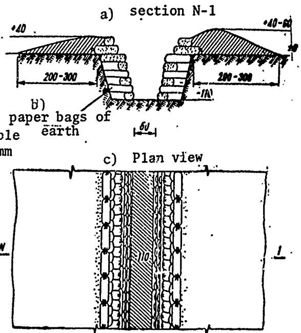
Figure 20 Revertment of trench slopes made from dirt filled bags. 10 running meters of trench require 20 manhours for revertment
