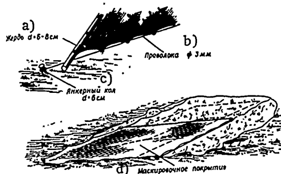
Figure 60 Camouflaging the entrance ramp with a removable blind. a) pole d = 6-8 cm; б) wire F 3 mm; в) anchor peg d = 6 cm; г) camouflage cover.
