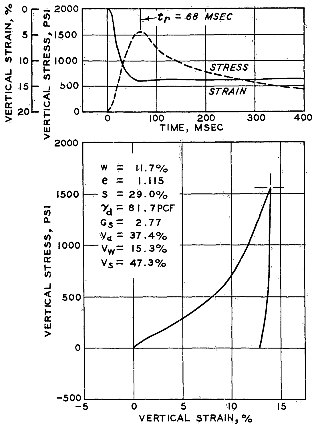
Fig. 6. Dynamic uniaxial strain test DP 1.1.3
