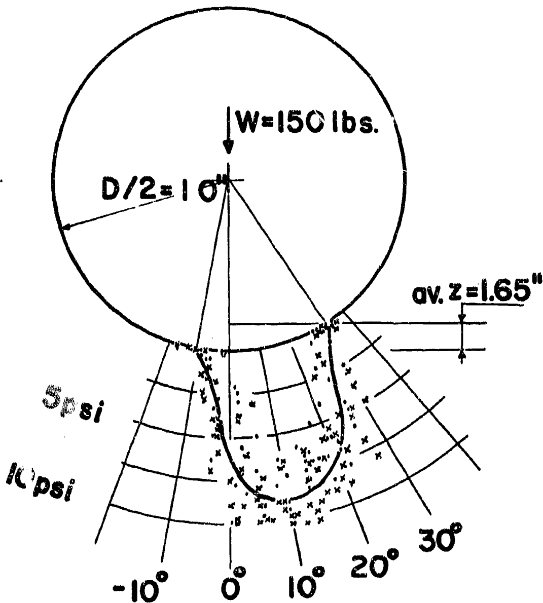
SPERPOSITION OF NORMAL PRESSURE DISTRIBUTION DIAGRAMS UNDER A 20x3" WHEEL IN SANDY-LOAM AT w=16.0\% with 150 lbs AXIAL LOAD.
