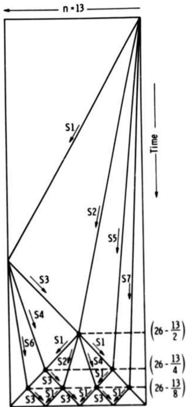
Fig. 2--A 2n-2 Solution for a Firing Squad of Length 13
