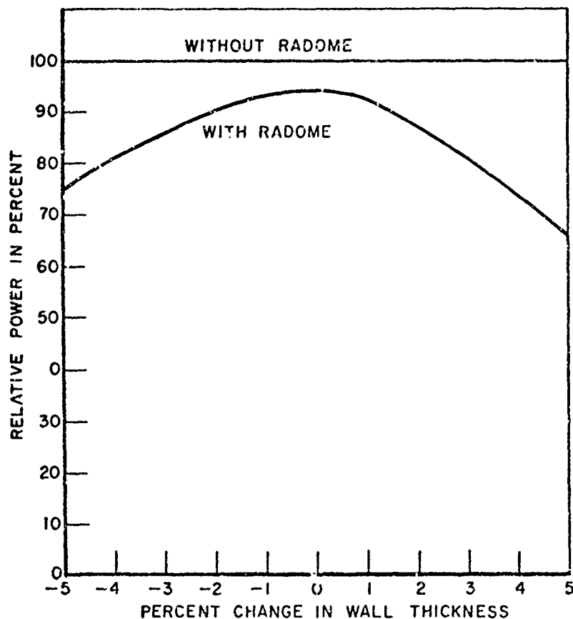
Fig. 11. On-axis transmission efficiency for pyroceram ogive radome with hemispheric nose cap as a function of its wall thickness. Perpendicular polarization at design frequency.
