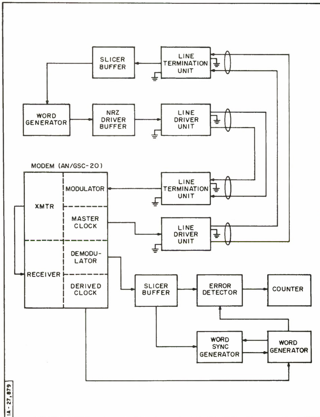
Figure 11. Baseband Data Transmission System Test Configuration
