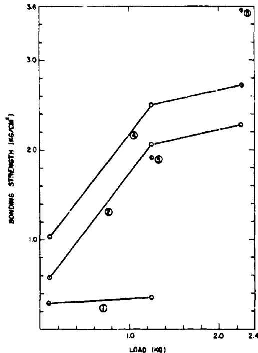
Figure 2. Mean bonding strength vs load, exerted for 60 min. Circled numbers indicate test conditions: 1. Polished cylinders placed together after 15 min in box. Saturated atmos. 2. Polished cylinders placed together immediately. Saturated atmos. 3. Cylinders with microtomed surfaces, placed together after 15 min in box. Relative humidity 100%. 4. Cylinders with microtomed surfaces, placed together after 15 min in box. Relative humidity near 0%.
