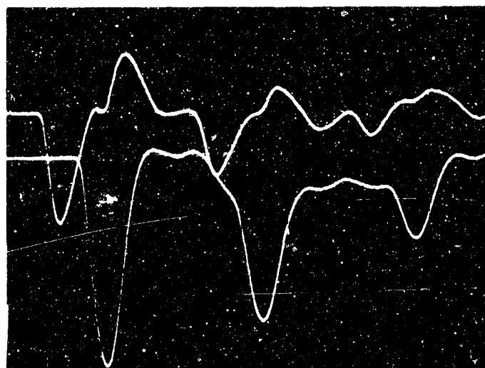
Fig. 27 - Propagation of stress pulse from polystyrene to clay
