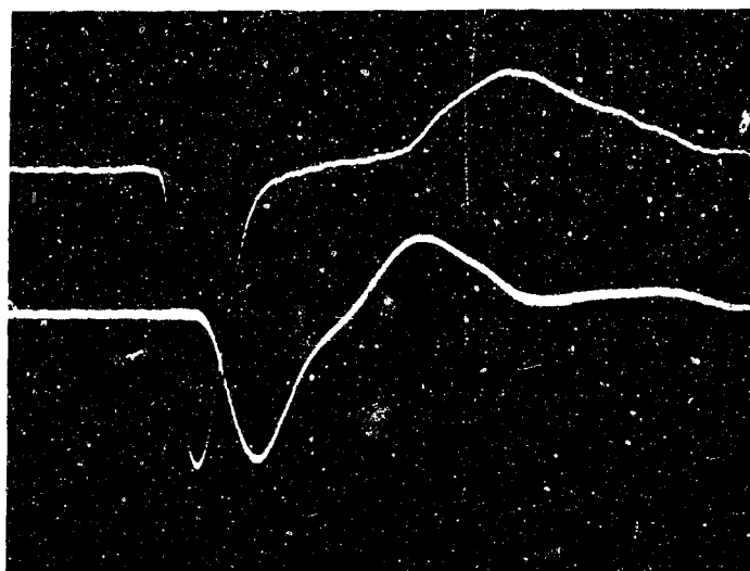
Fig. 29 - Recording of transmitted pulse in clay by two strain gages mounted 8 cm apart
