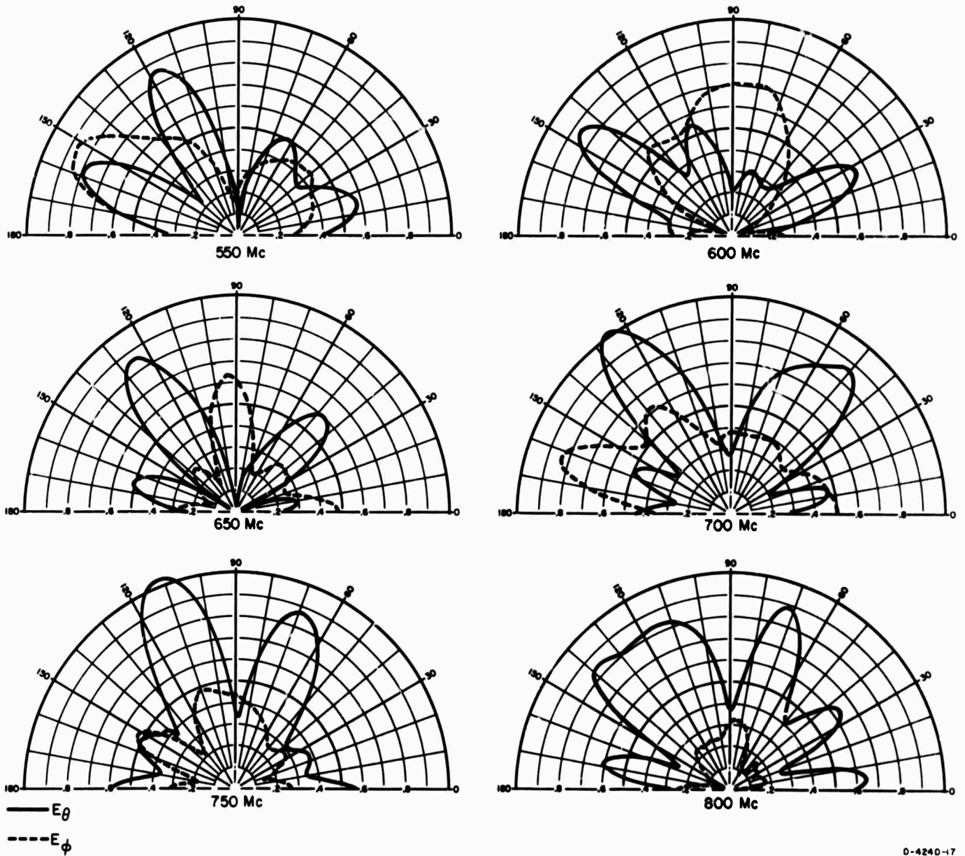
FIG. 6(d) ELEVATION PLANE PATTERNS OF A SHORT SLOPING WIRE ( 0.076\lambda-0.203\lambda ) FED AGAINST A CONICAL METALLIC GROUND FOR \phi = 0^\circ , SLOPE ANGLE = 45^\circ , CONE ANGLE FROM HORIZON = 25^\circ
