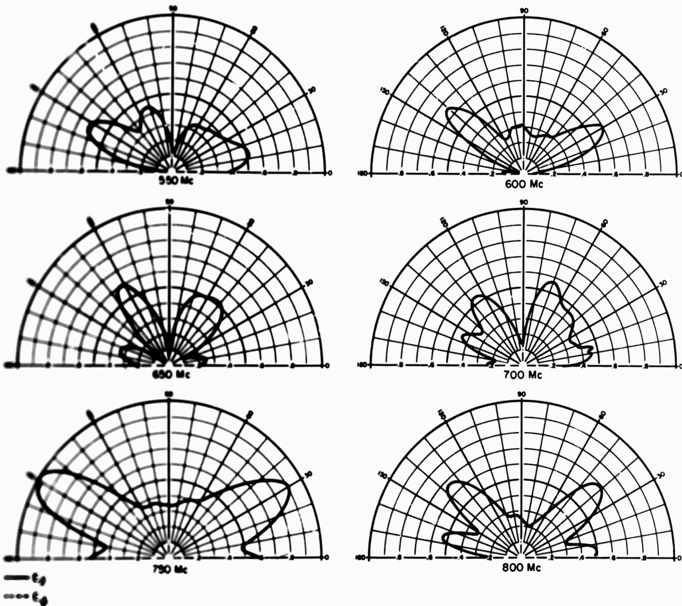
FIG. 5(e) ELEVATION-PLANE PATTERNS OF A SHORT SLOPING WIRE ( 0.076\lambda - 0.203\lambda ) FED AGAINST A PLANE METALLIC GROUND FOR \phi = 0^\circ AND SLOPE ANGLE = 30^\circ
