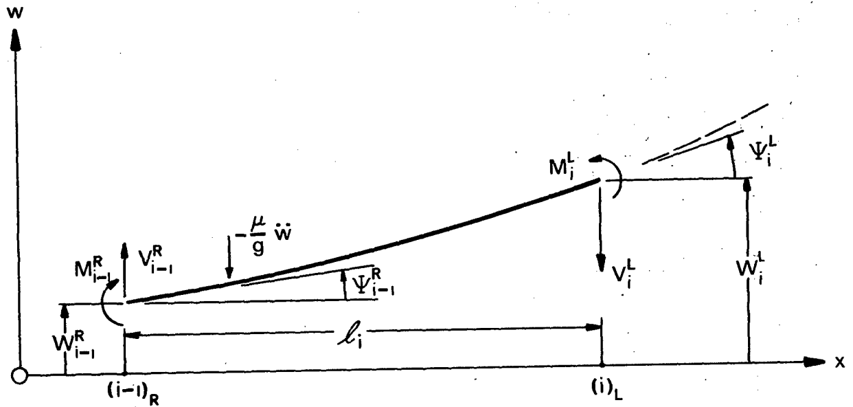
Forces and Deflections for Beam Element
