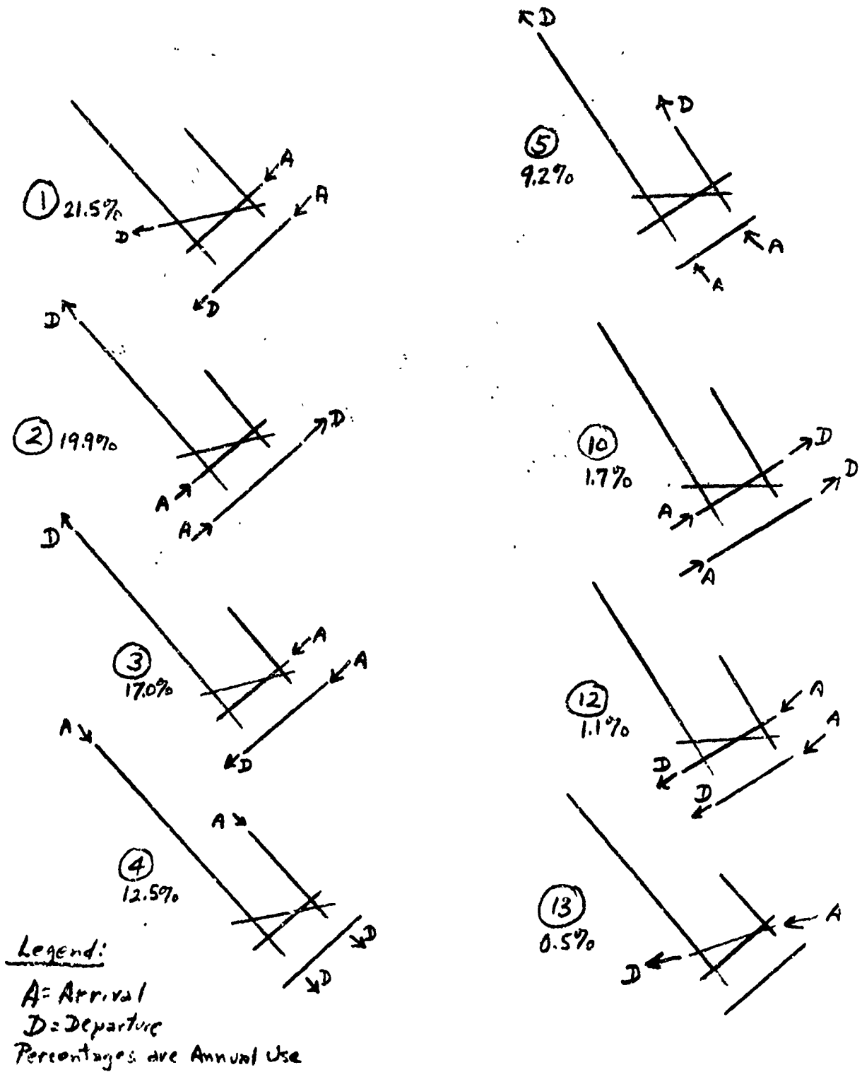
Figure II-1. VFR Runway Use Combinations
