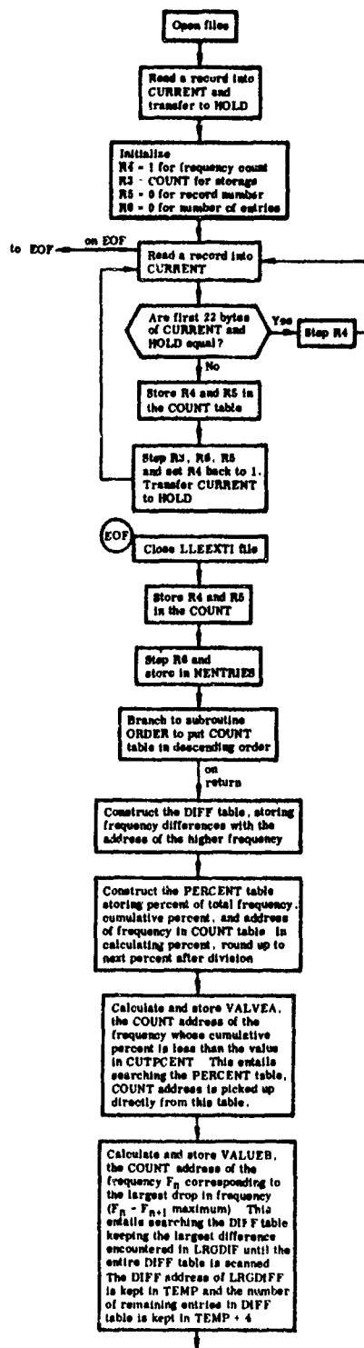
Fig. 4 Flow Diagram for EXTRACT Program
