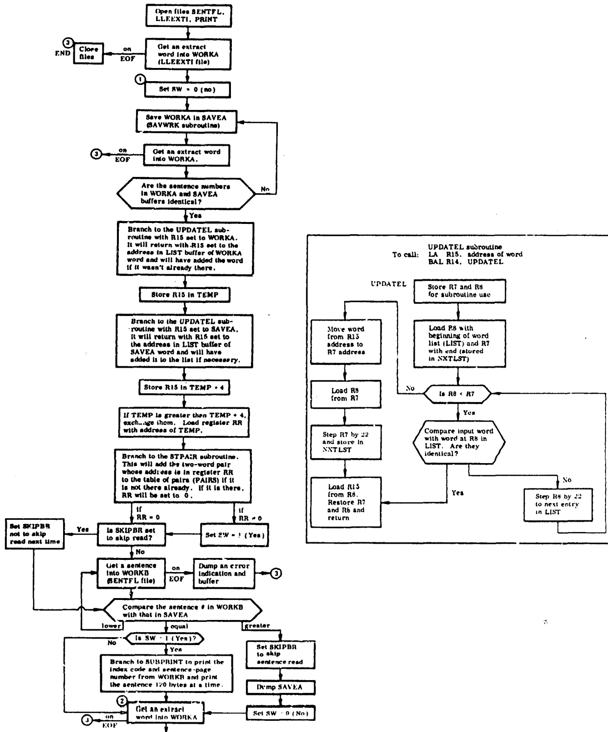
Fig. 5 Flow Diagram for PRNTEXT Program
