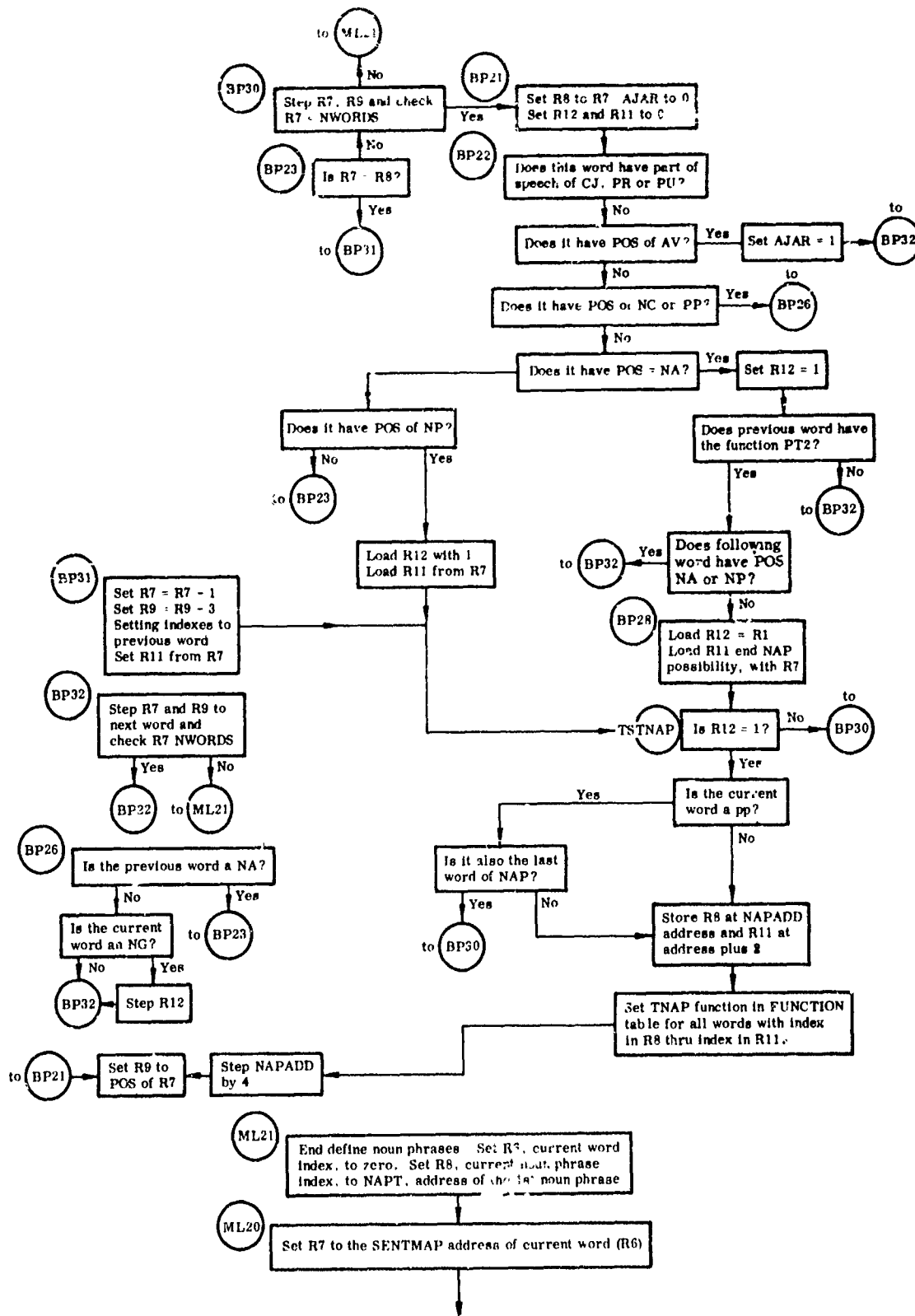
Fig. 8 MEDLIST Detailed Flow Diagram (Cont.)
