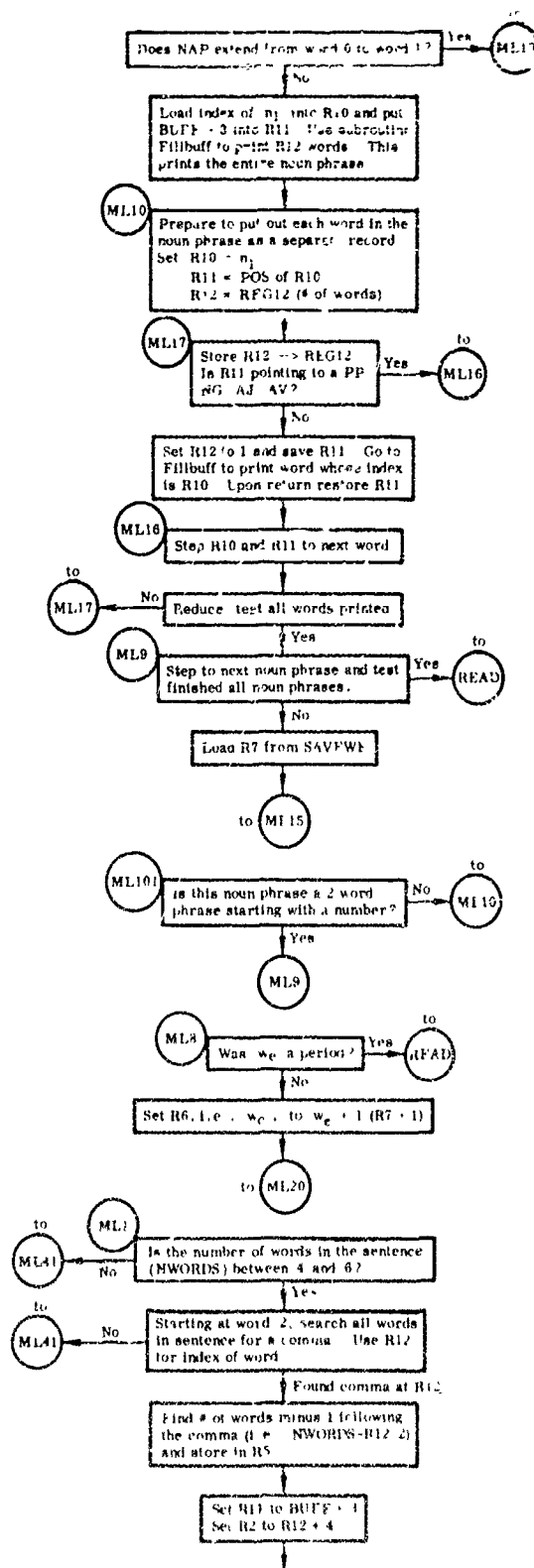
Fig. 8 MEDLIST Detailed Flow Diagram (Cont.)
