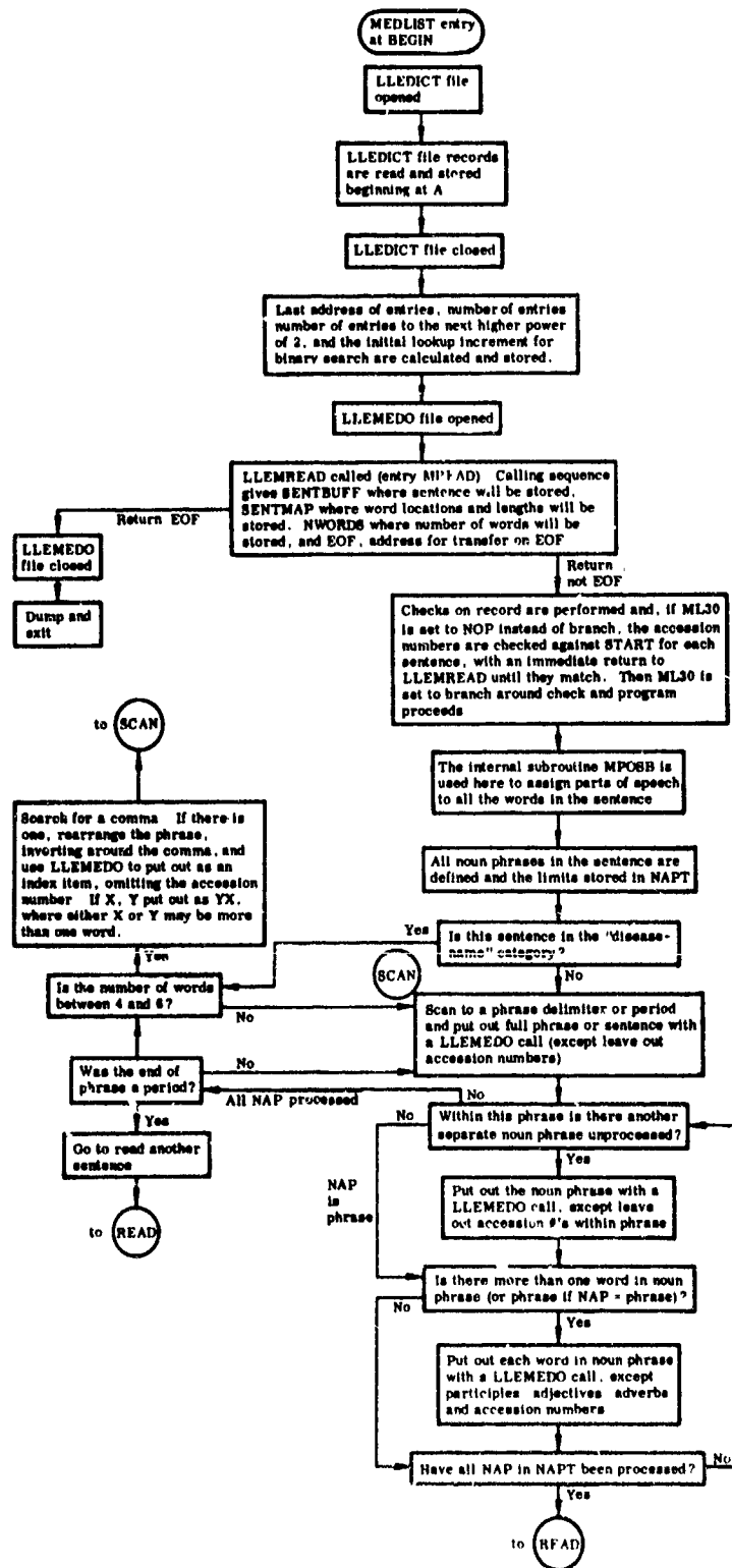
Fig. 6 Overall MEDLIST Operation
