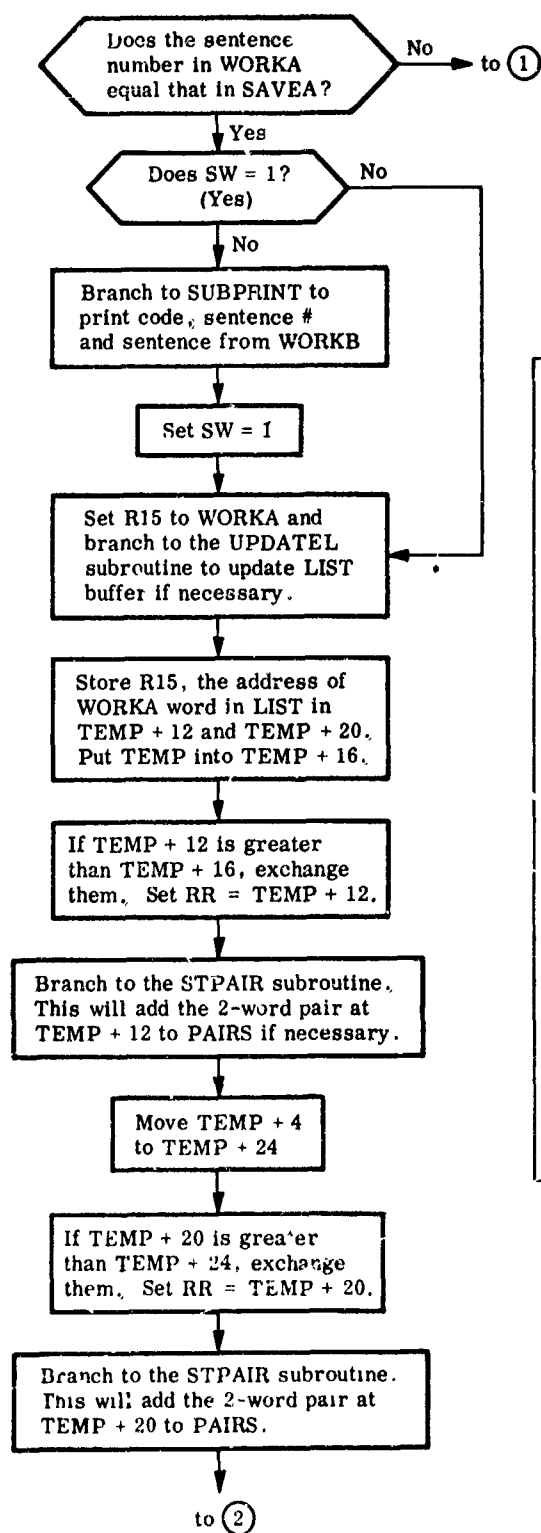
Fig. 5 Flow Diagram for PRNTEXT Program (Cont.)
