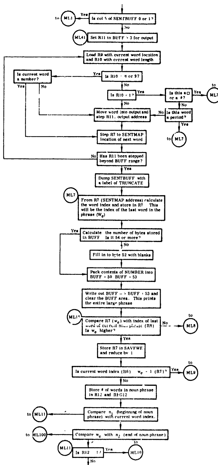
Fig. 8 MEDLIST Detailed Flow Diagram (Cont.)
