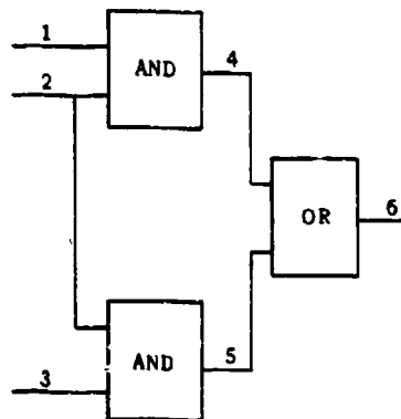
Fig. 1 - Two-input AND gate with associated singular cover and D -cube
