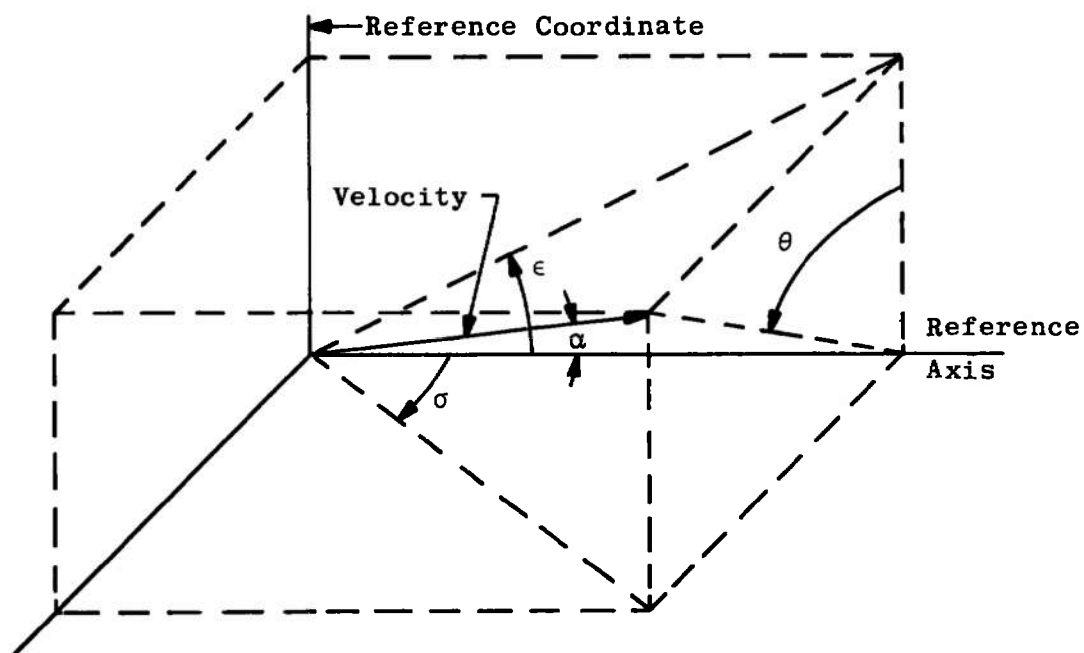
Fig. 1 Cone-Probe and Flow Field Nomenclature
