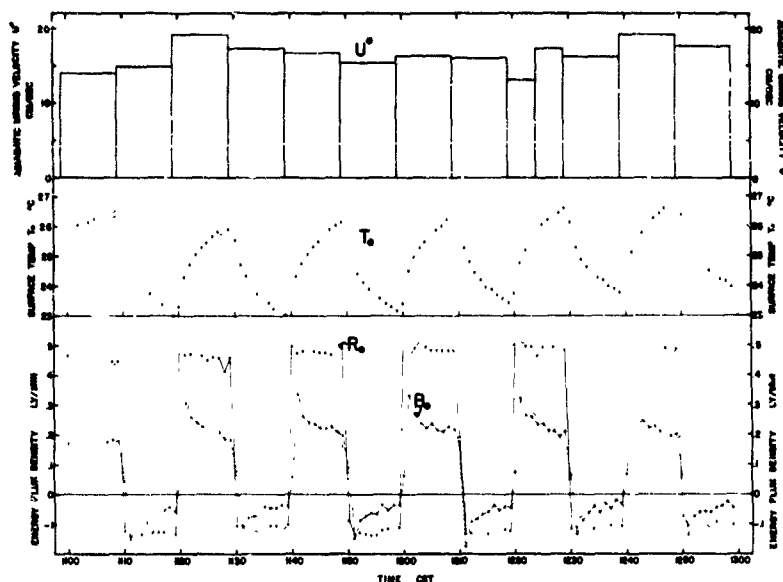
Fig. 4. Data plotted for Run 2, Sept. 2, 1965; six 20 minute periods. A_0 by eddy diffusion measurement was not available. B_0 here was obtained by the combination temperature integral-flux plate method.
