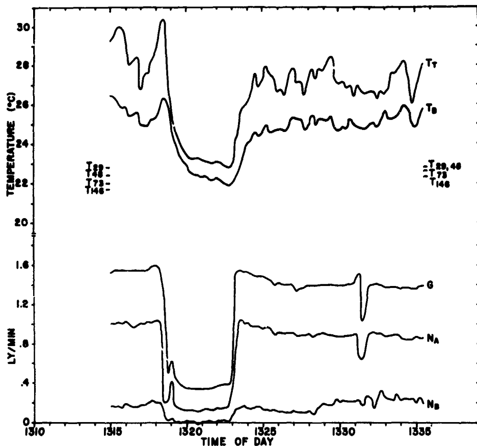
Fig. 5. Data sequence, 20 July 1966. T_T and T_B temperature at top and bottom of canopy, G = global radiation, N_A and N_B net radiation above and below canopy.
