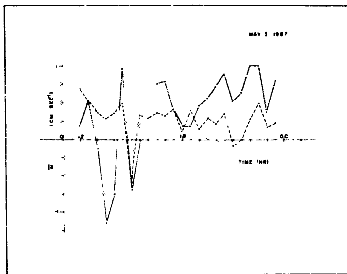
Fig. 4.1. The time series of vertical velocity ( \bar{w} ) at 320 cm (computed from top level divergence only) is shown for two cases on 3 May: 1) Mast 1 wind direction used at all masts (solid line), and 2) Individual mast direction used (broken line).
