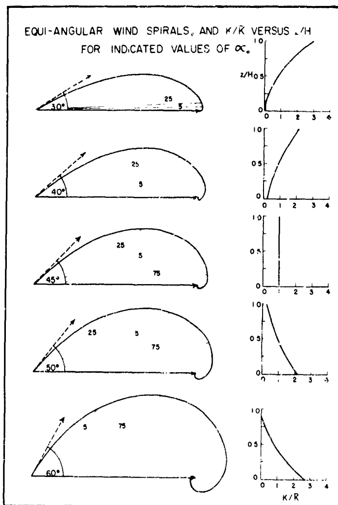
Fig. 2. A family of equi-angular wind spirals and corresponding vertical profiles of eddy diffusivity ( K relative to \bar{K} , versus z/H where H = geostrophic wind level), for five selected values of \alpha_0 (angle between surface stress and ambient flow). The special case of the Ekman spiral is illustrated at the center.
