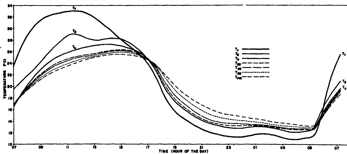
Fig. 8. Diurnal sequence of canopy and air temperatures on 30 and 31 July, 1966.
