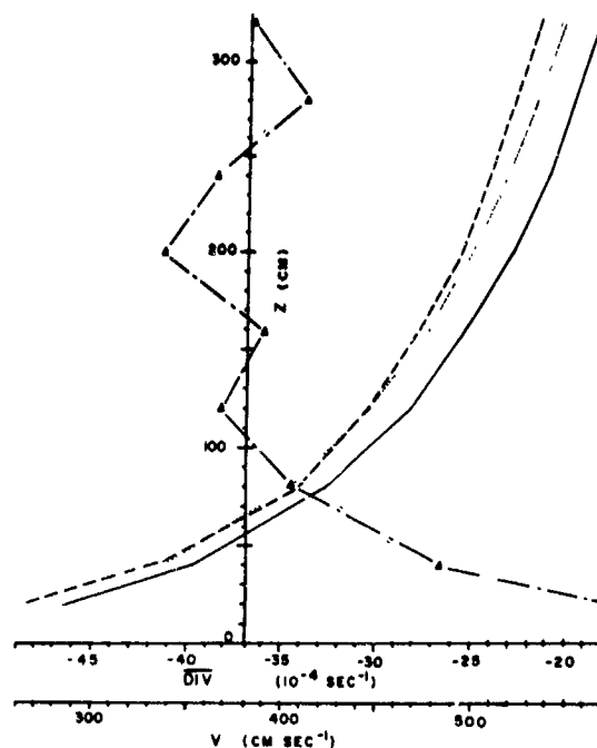
Fig. 3.4 . Vertical profiles of windspeed ( V , solid line is mast 1, dashed line is mast 2, and dotted line is mast 3), and the resulting divergence (dash-dot line) for one-half hour period (1631-1700 May 4) which was representative of most other times.
