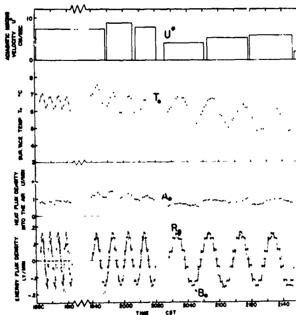
Fig. 5a. (Continued on following page) Data plotted for Run 7, night of Oct. 27-28, 1965. Sequence of periods (in minutes) was: 5-5-5-5, 10-10-10-10, 20-20-20-20, 40-40-40 and 5-5-5-5. A_0 obtained by eddy diffusion equation, B_0 by combination temperature integral-flux plate method.
