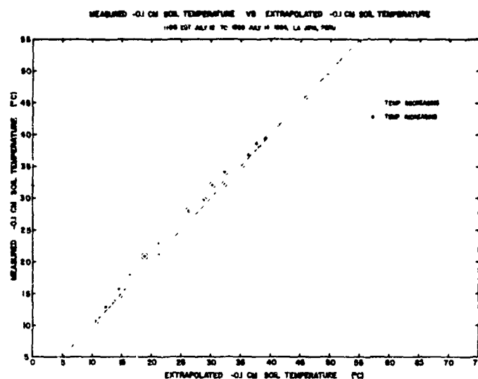
Fig. 6. Ten min mean soil temperature at the nominal depth of -0.1 cm as measured by an 0.001 mil nickel wire resistance thermometer versus the temperature determined by the extrapolation of one minute sub-soil temperatures to -0.1 cm and then averaged for 10 min periods. Allowance was not made for phase lags in the extrapolated sub-soil temperatures.
