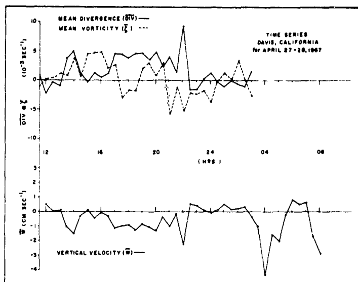
Fig. 3.1. The time series of mean divergence mean vertical velocity computed from the divergence and mean vorticity (broken line) at the 320 cm level for the period 27-28 April 1967 at Davis, California.
