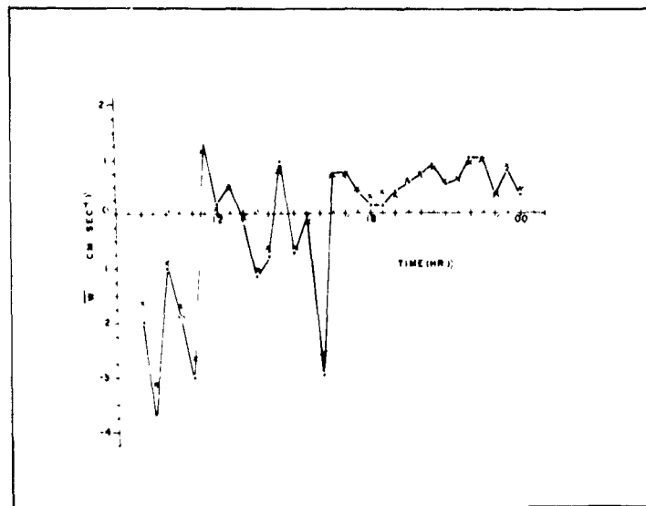
Fig. 3.3. A time series of vertical velocity at the 320 cm level. Two methods were used: 1) top divergence only (solid line), and 2) two-level divergence averages (shown by x's with no connecting line).
