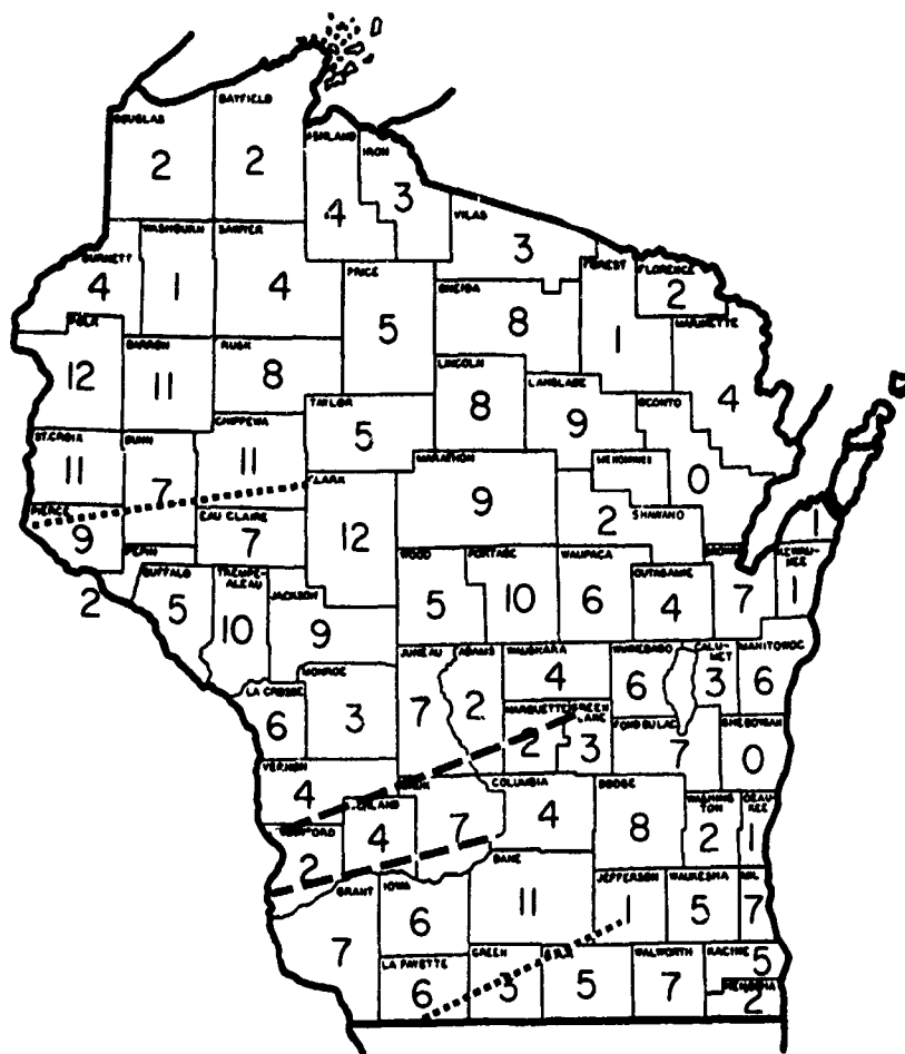
Fig. 4. Number of reported tornadoes by county, 1916-1964 (after Burley and Waite, 1965). Superimposed lines (short dashes for "alleys" A and D, and long dash for "shunted areas" B and C) indicate paths chosen for investigation.
