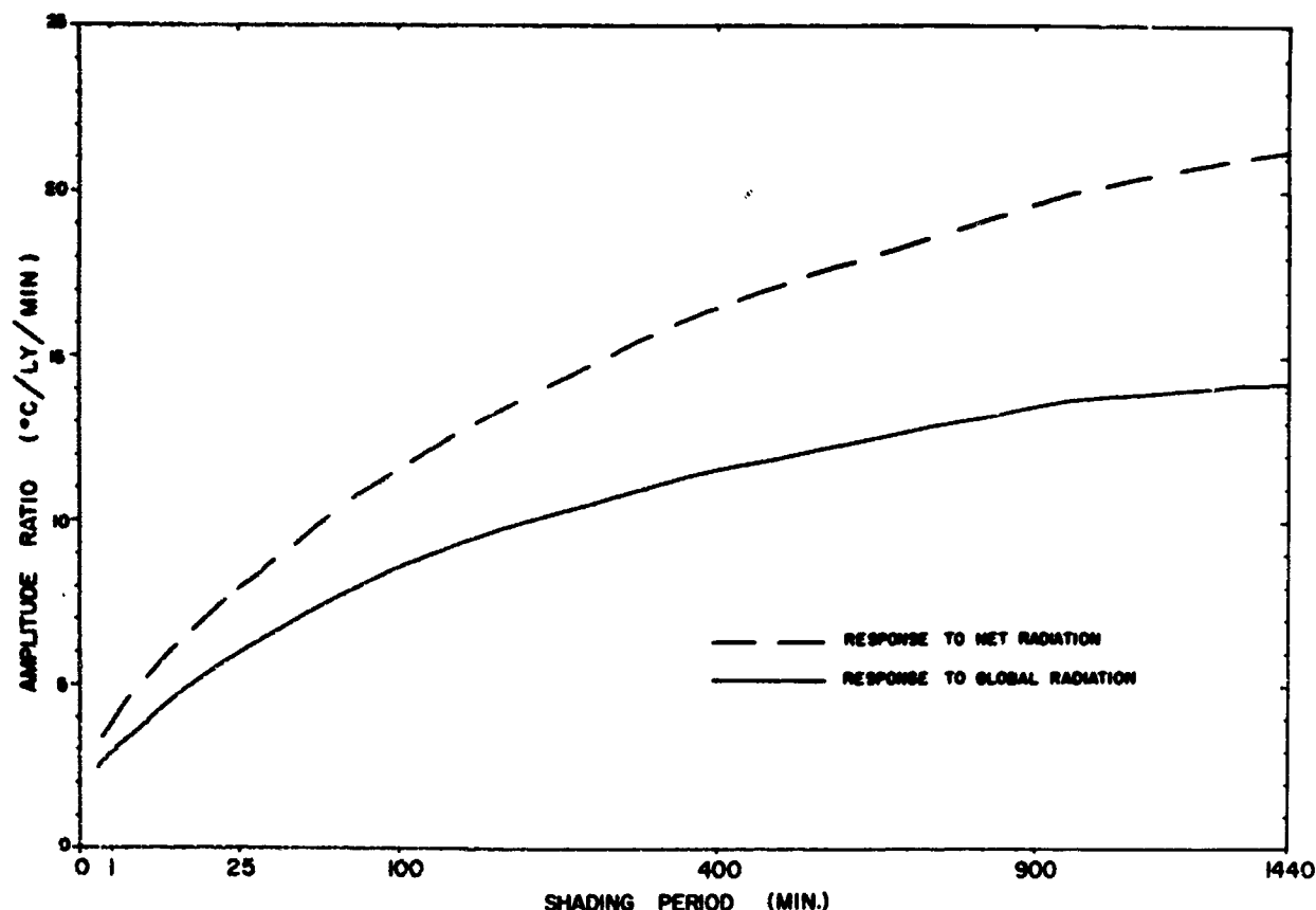
Fig. 9. Thermal response of the canopy surface to global radiation and net radiation for afternoon observations of 20 July 1966.
