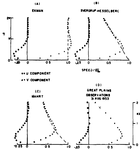
Fig. 2.1. Comparison of three steady-state boundary layer wind models for latitude 42.5^\circ \text{N} with data from the Great Plains Turbulence Field Program. Coordinates aligned with V-component of wind parallel to mean geostrophic wind direction. Dashed lines indicate mean geostrophic wind profile.
