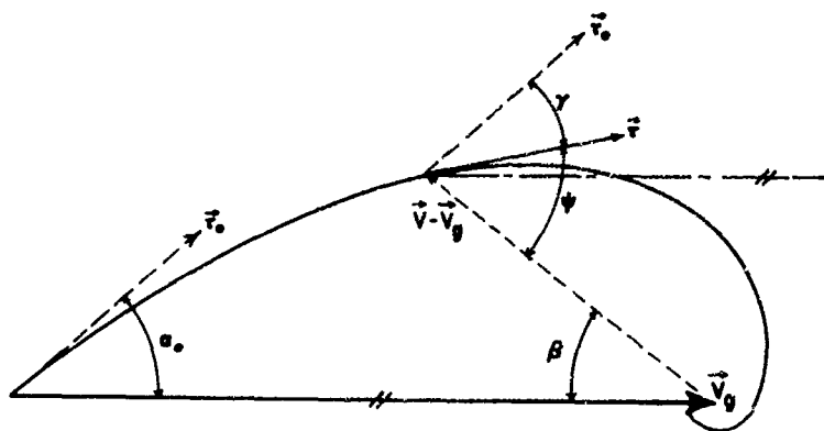
Fig. 1. Representative planetary boundary layer wind spiral depicting the vectors of shear stress ( \tau ), and the angular quantities \alpha_0 , \beta , \gamma and \psi .
