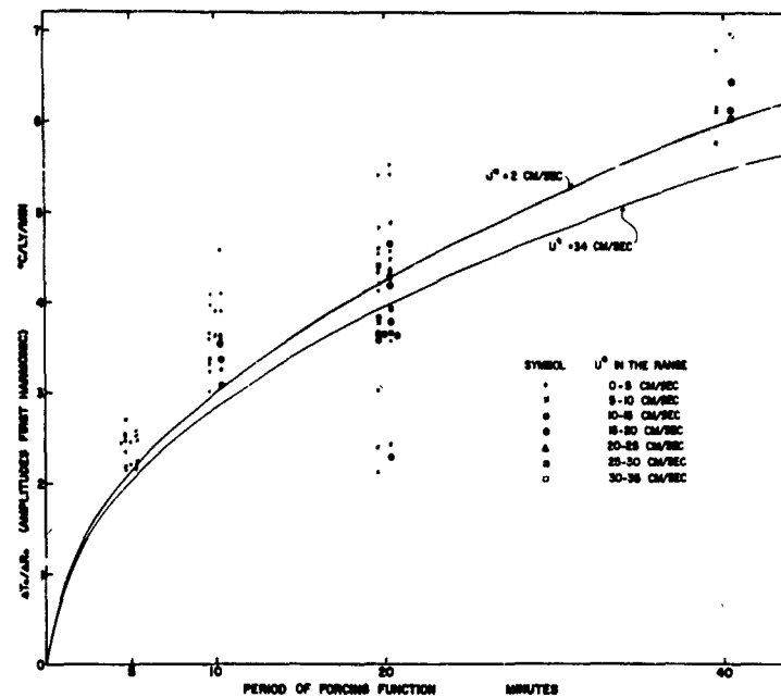
Fig. 6. Based on R_0 , model predictions (smooth curves) and observed values of thermal response, first harmonic only, for all periods (except the first one in each daytime run) of all nine runs. For greater clarity, the points are spread laterally; variability of that amount is not implied for the lengths of the 5, 10, 20 and 40 minute runs.
