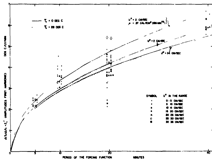
Fig. 7. Based on F_0 , model predictions (smooth curves) and observed values of thermal response, first harmonic only, for all periods (except the first one in each daytime run) of all nine runs. The upper smooth curve is for a thermal admittance which is 12% less than was first estimated, in an effort to get a better fit for the data.
