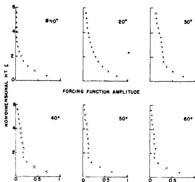
Fig. 3.1. Profiles of forcing function amplitude for ten-degree latitude increments. Nondimensional height \zeta = \sqrt{f/K} Z .
