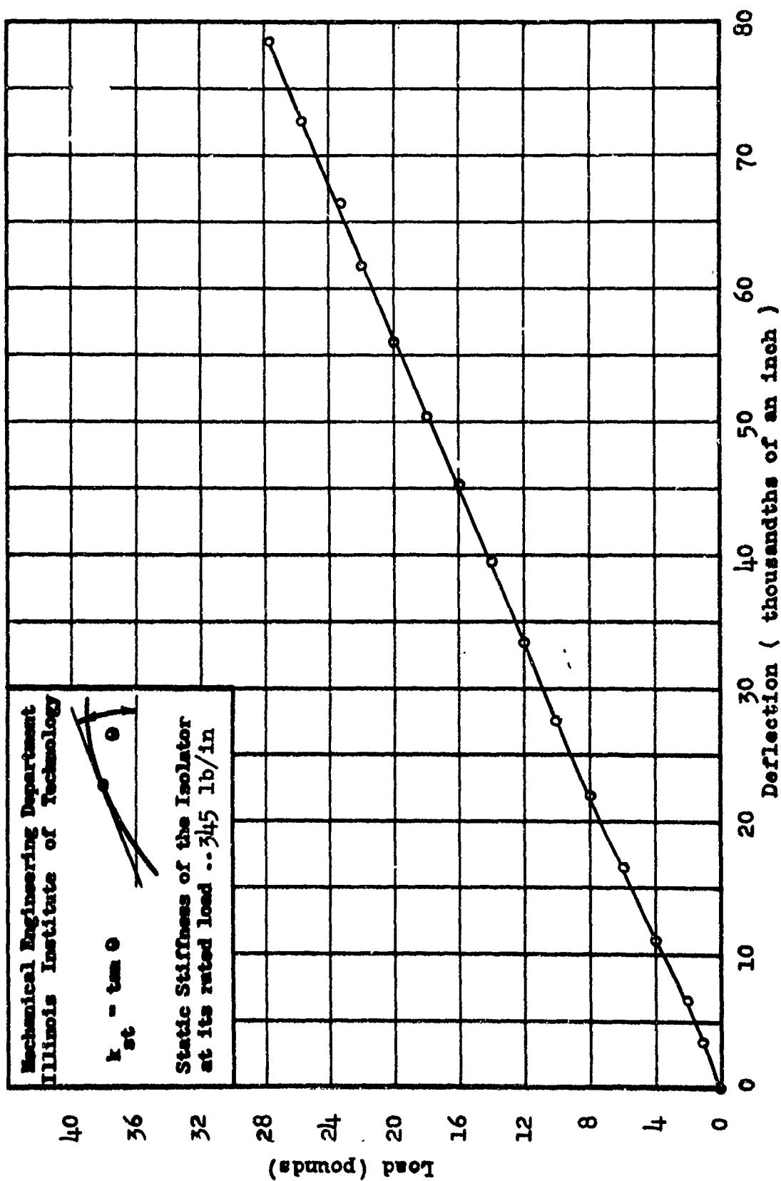
Load-Deflection Curve - Barry 104-20
