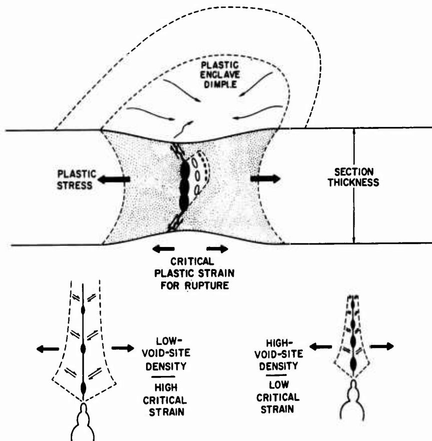
Fig. 47 - Features of high-ductility plane stress fracture as illustrated by through-thickness contraction and the development of plastic enclave dimpling. The intrinsic void site density quality of the steel determines the critical plastic strain for rupture. Accordingly, metallurgical quality controls the degree of contraction, the dimple size, and the measured level of fracture toughness.
