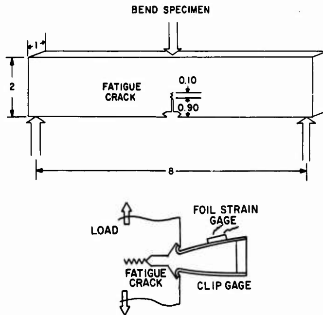
Fig. 45 - General features of bend-type K_{Ic} test specimens. The clip gage detects the first signs of elastic fracture instability or of crack blunting.
