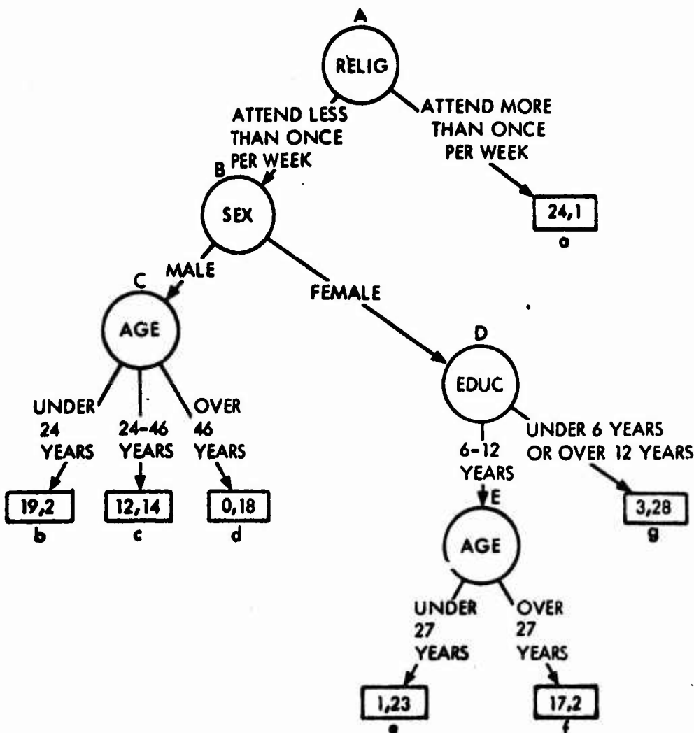
Figure 4. Sample Decision Tree From Watts Riot Data
